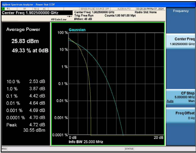
Band2-15MHz-QPSK-19125-75RB#0
