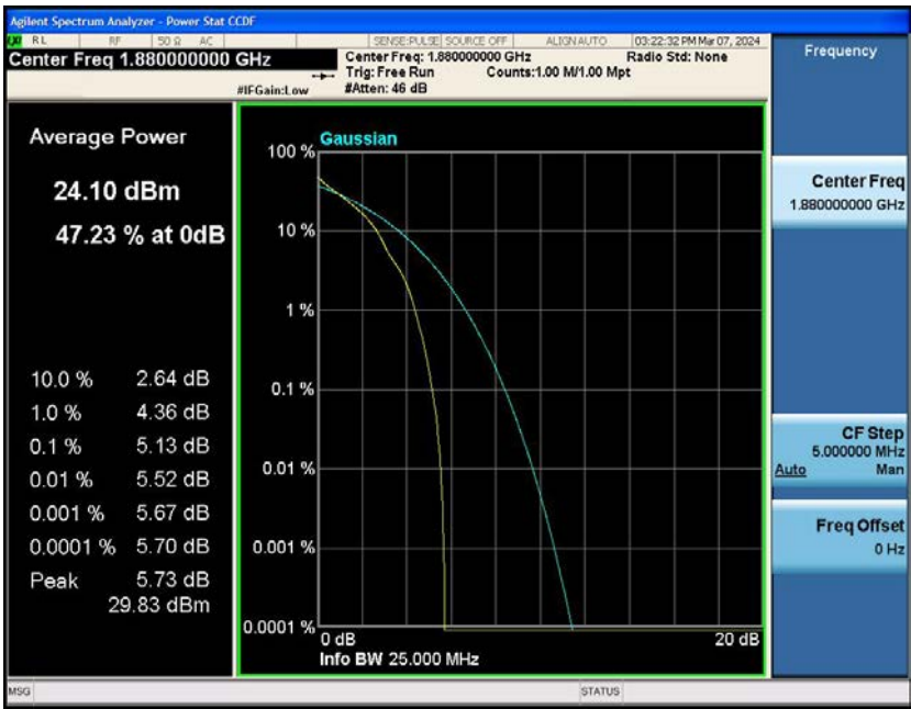
Band2-3MHz-QPSK-18900-15RB#0
