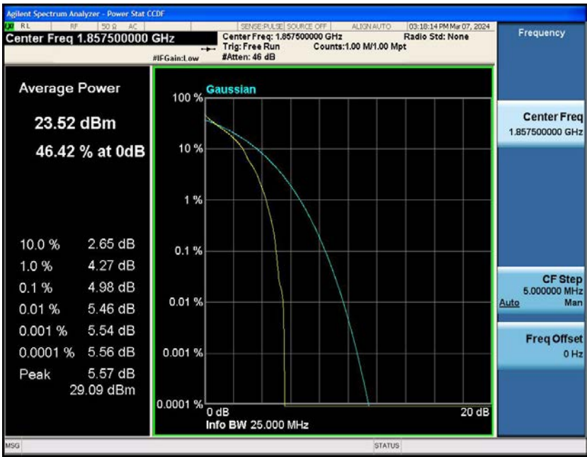
Band2-15MHz-QPSK-18675-75RB#0
