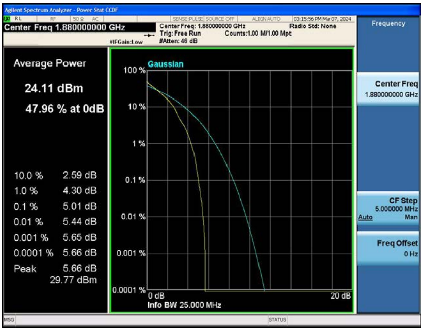
Band2-1.4MHz-QPSK-18900-6RB#0
