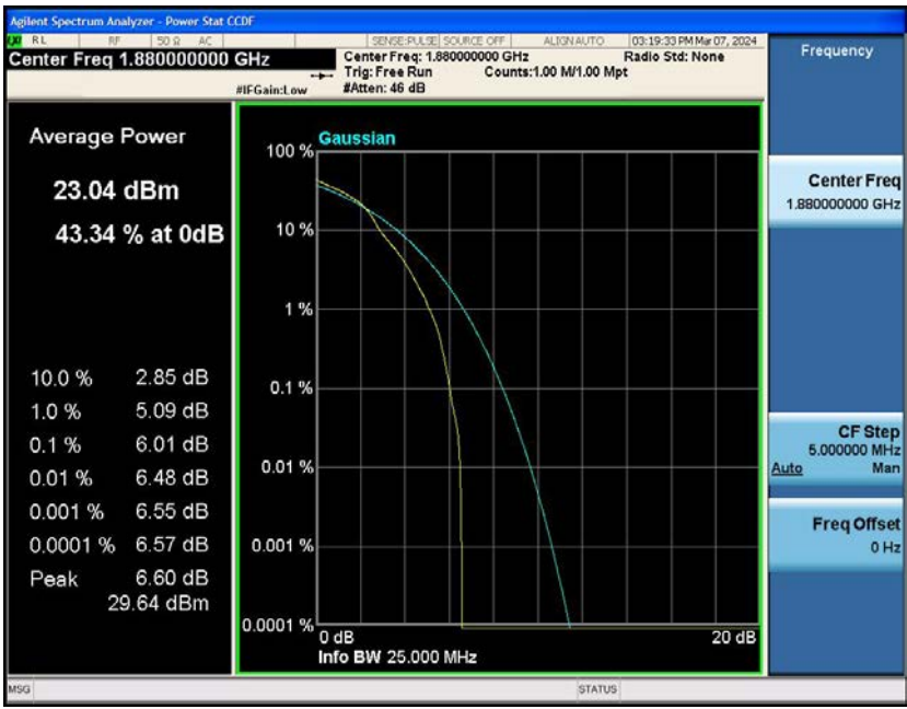
Band2-15MHz-16QAM-18900-75RB#0
