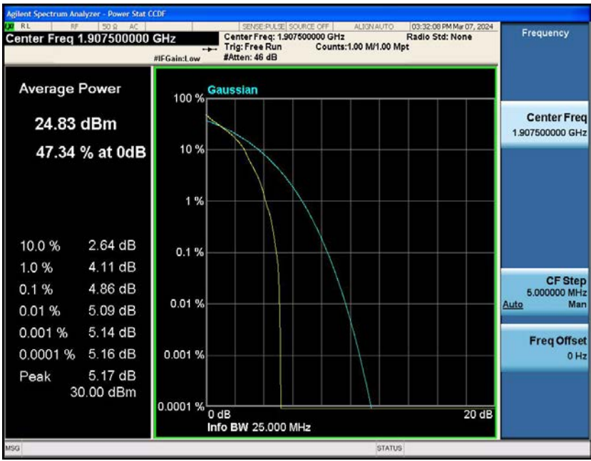
Band2-5MHz-QPSK-19175-25RB#0
