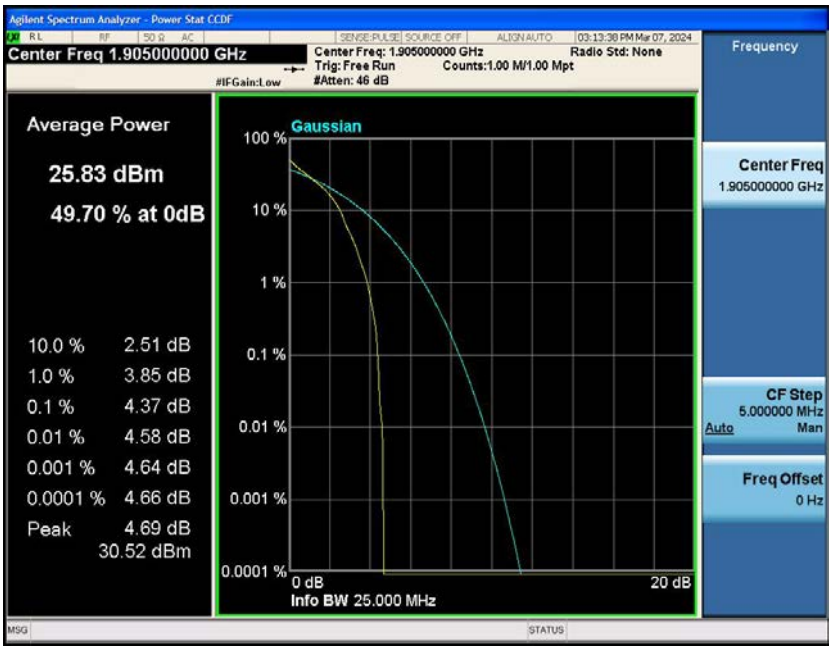
Band2-10MHz-QPSK-19150-50RB#0
