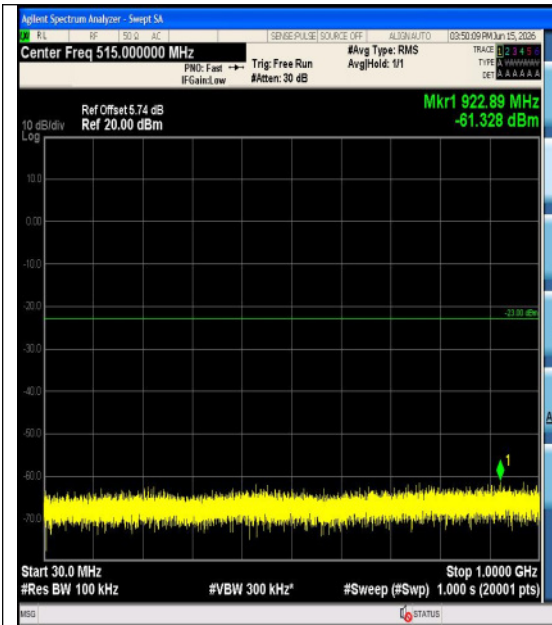
Band2-10MHz-QPSK-18650-1RB#0-3000~2000 0-PASS
