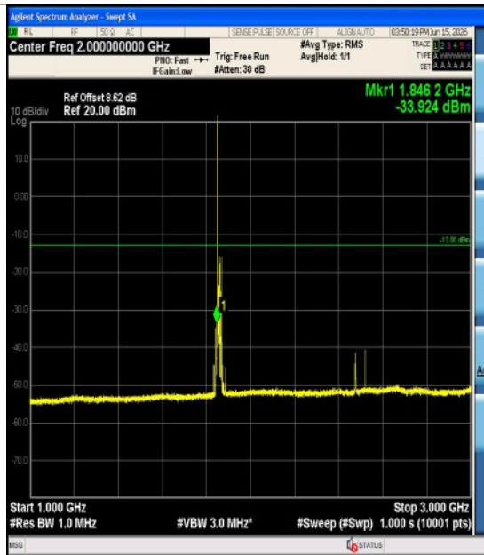
Band2-10MHz-QPSK-18650-1RB#49-0.009~0.1 5-PASS
