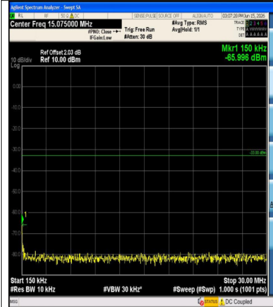
Band2-5MHz-16QAM-19175-25RB#0-1000~300 0-PASS
