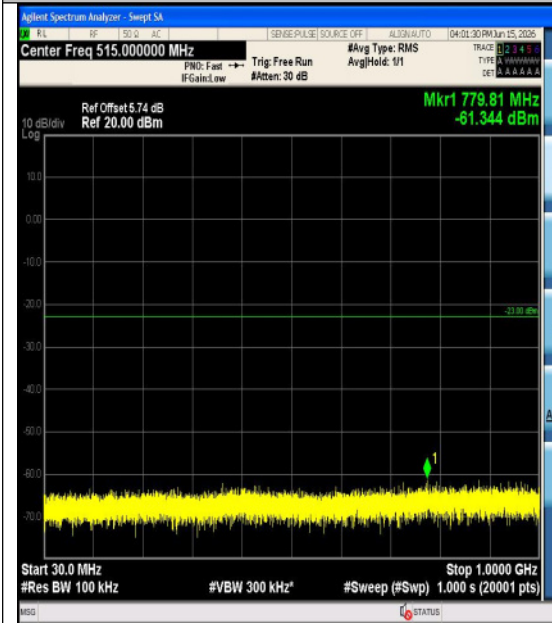
Band2-10MHz-QPSK-19150-1RB#0-3000~2000 0-PASS
