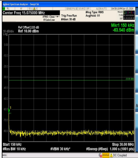
Band2-15MHz-QPSK-18675-1RB#74-1000~300 0-PASS
