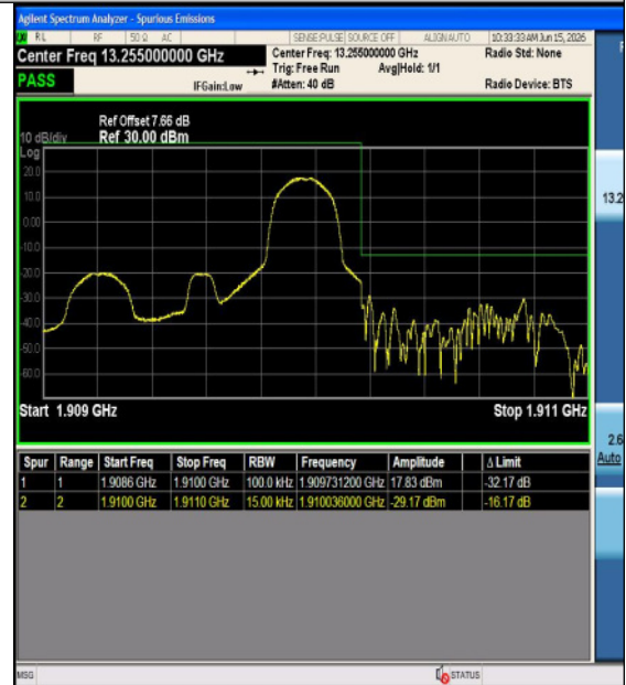
Band2-1.4MHz-16QAM-19193-1RB#0-PASS
