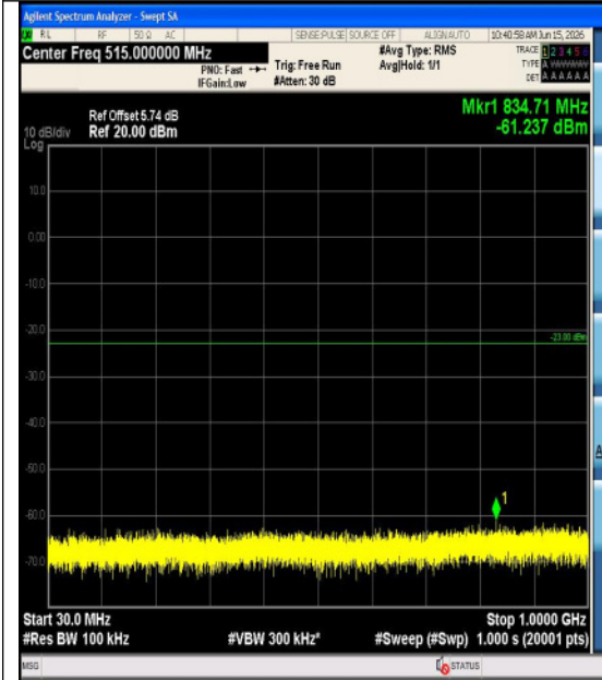
Band2-1.4MHz-16QAM-18607-1RB#5-3000~200 00-PASS
