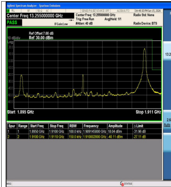
Band2-15MHz-16QAM-19125-1RB#0-PASS
