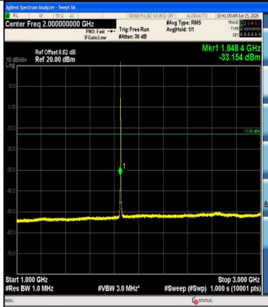
Band2-1.4MHz-16QAM-18607-6RB#0-0.009~0.1 5-PASS
