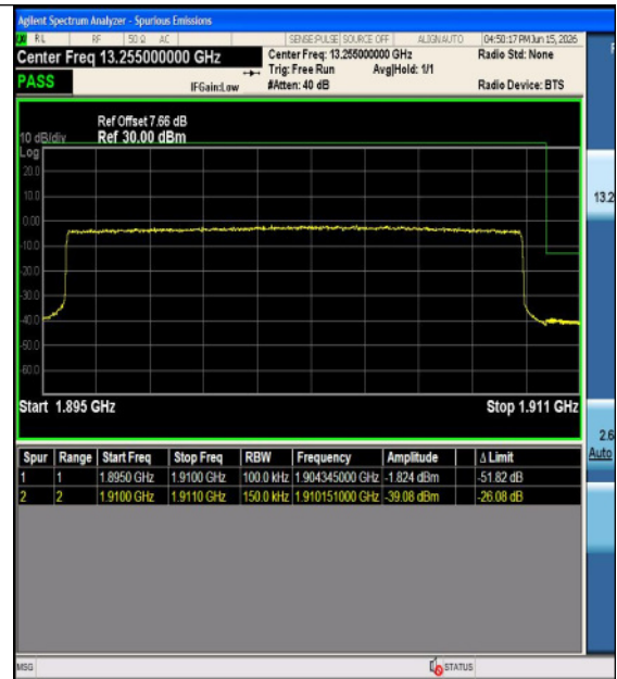
Band2-15MHz-16QAM-19125-1RB#74-PASS
