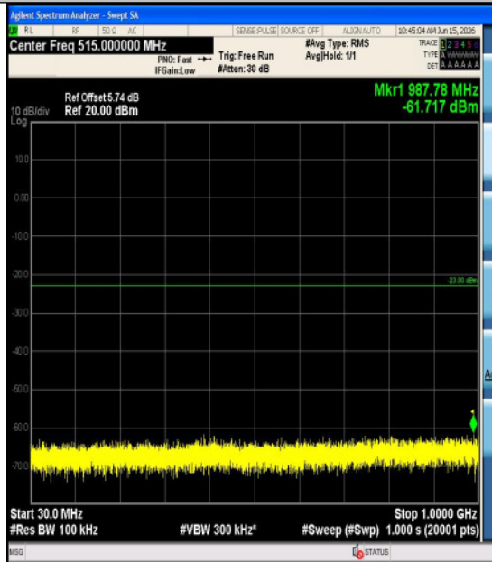
Band2-1.4MHz-16QAM-18900-1RB#0-3000~20000 00-PASS
