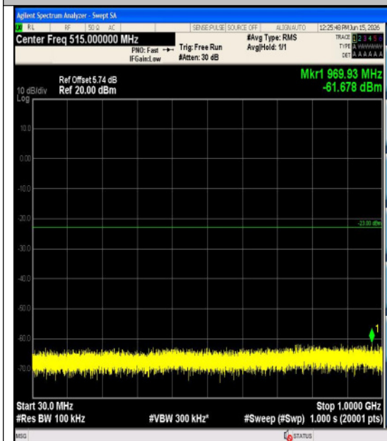
Band2-3MHz-QPSK-18615-15RB#0-3000~2000 0-PASS
