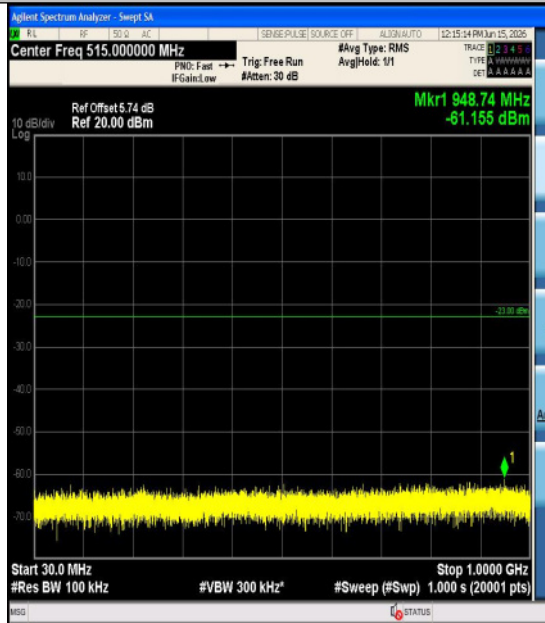
Band2-3MHz-16QAM-18615-1RB#0-3000~2000 0-PASS
