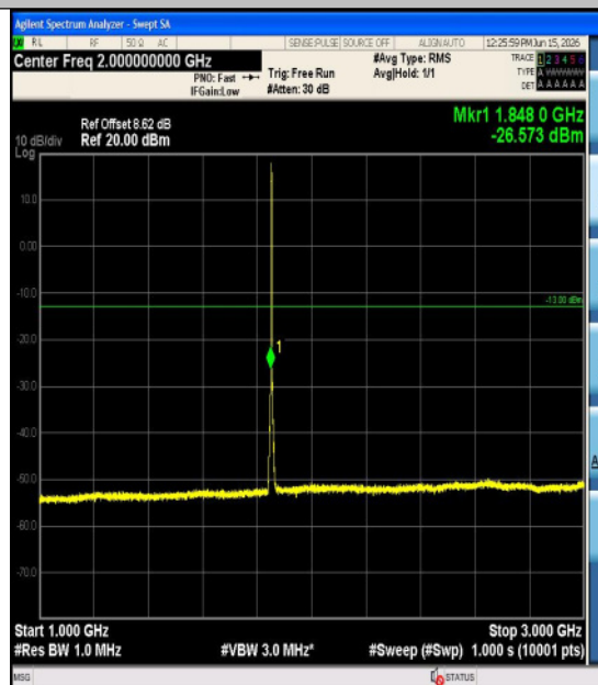
Band2-3MHz-16QAM-18615-1RB#0-0.009~0.15-PASS
