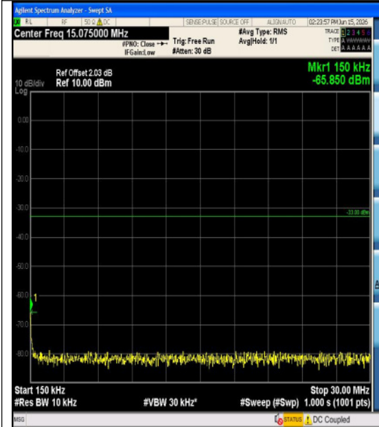
Band2-5MHz-16QAM-18900-1RB#0-1000~3000-
