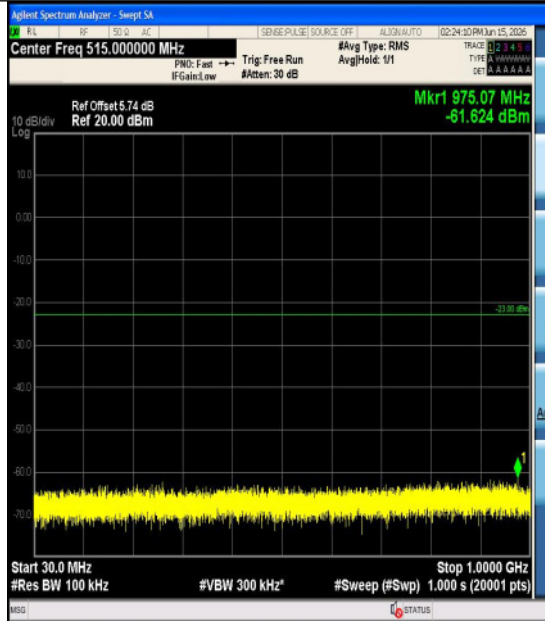
Band2-5MHz-16QAM-18900-1RB#0-3000~2000
