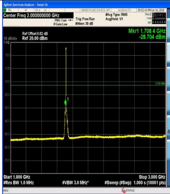
Band4-10MHz-16QAM-20000-1RB#0-0.009~0.1 5-PASS
