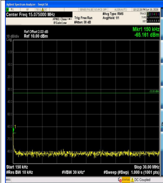
Band4-15MHz-QPSK-20025-1RB#0-1000~3000-
