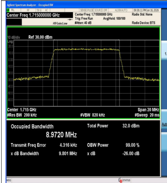
Band4-10MHz-QPSK-20175-50RB#0-PASS
