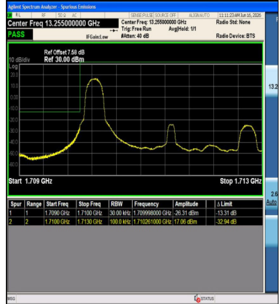
Band4-3MHz-16QAM-19965-15RB#0-PASS
