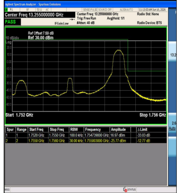
Band4-3MHz-16QAM-20385-1RB#0-PASS
