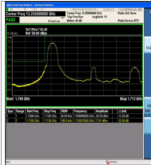
Band4-3MHz-QPSK-19965-15RB#0-PASS
