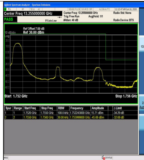
Band4-3MHz-16QAM-20385-15RB#0-PASS
