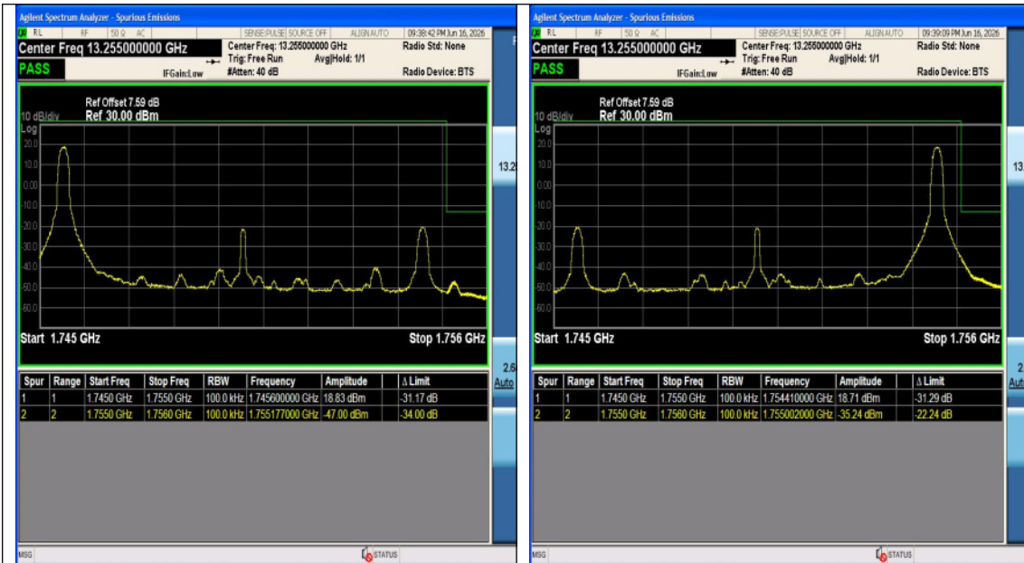
Band4-15MHz-QPSK-20025-1RB#0-PASS
