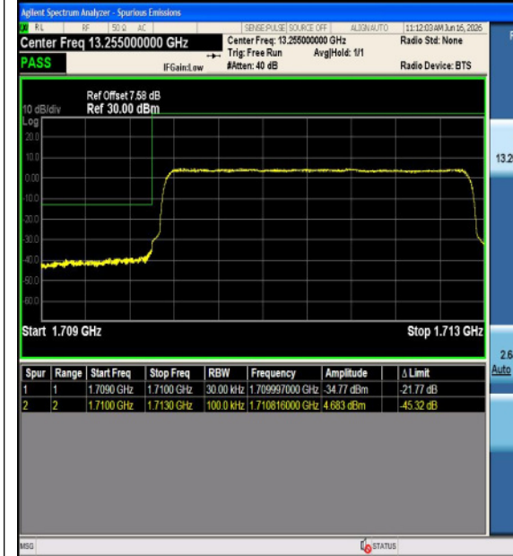
Band4-3MHz-16QAM-19965-1RB#14-PASS
