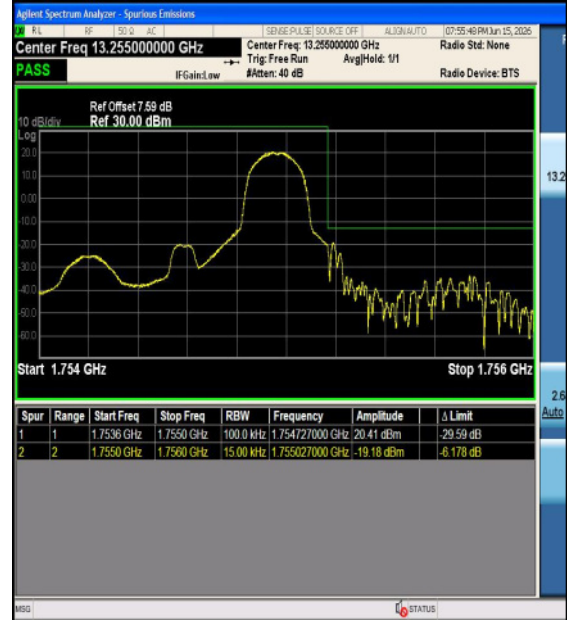
Band4-1.4MHz-16QAM-20393-1RB#0-PASS
