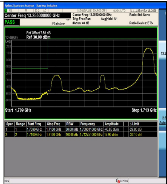
Band4-3MHz-16QAM-19965-1RB#0-PASS
