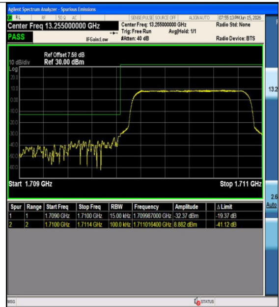
Band4-1.4MHz-QPSK-20393-1RB#5-PASS
