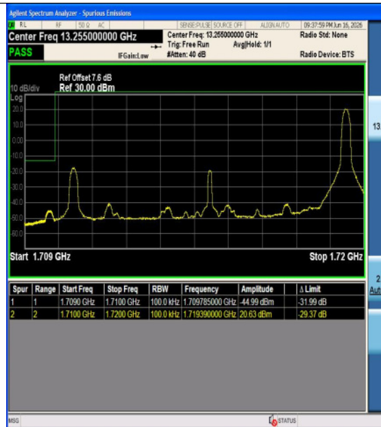
Band4-10MHz-16QAM-20000-1RB#0-PASS
