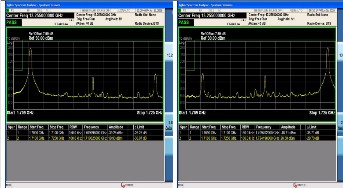
Band4-15MHz-QPSK-20025-75RB#0-PASS
