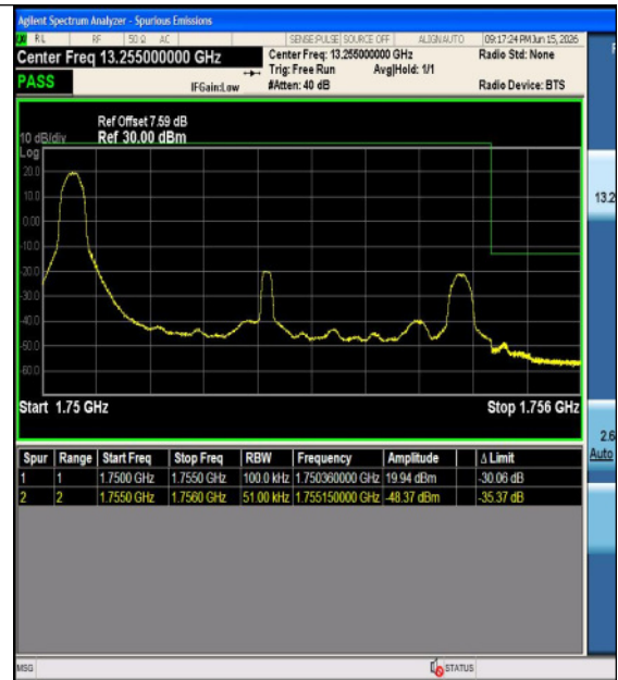
Band4-5MHz-16QAM-20375-25RB#0-PASS
