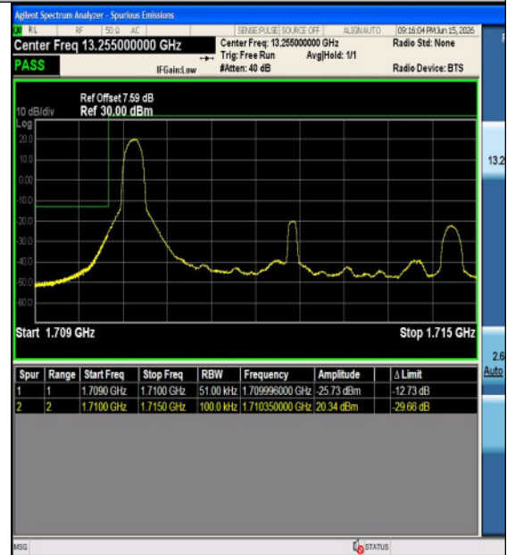
Band4-5MHz-16QAM-19975-25RB#0-PASS
