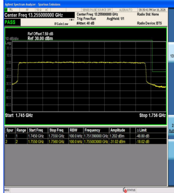
Band4-10MHz-16QAM-20350-1RB#49-PASS
