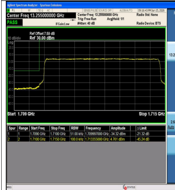
Band4-5MHz-16QAM-19975-1RB#24-PASS
