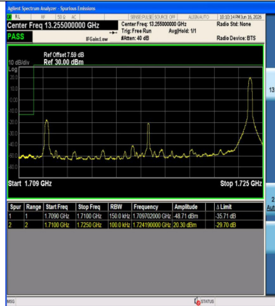
Band4-15MHz-16QAM-20025-1RB#0-PASS
