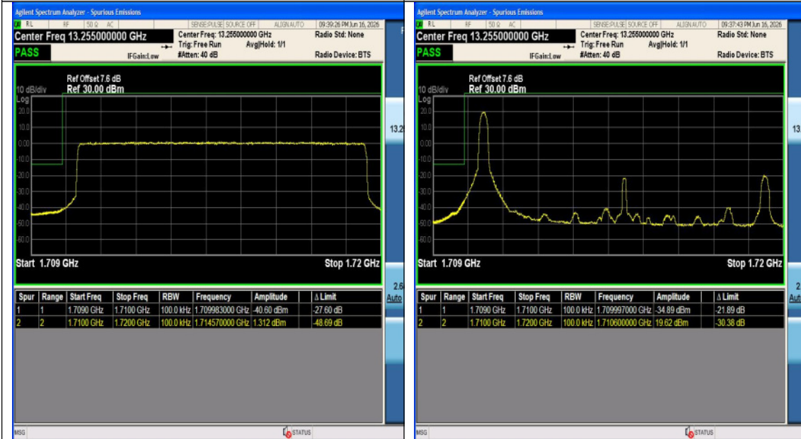
Band4-10MHz-16QAM-20000-1RB#49-PASS
