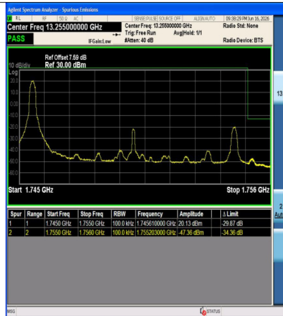
Band4-10MHz-QPSK-20350-50RB#0-PASS
