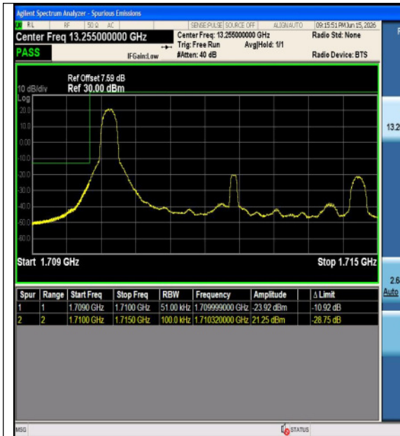
Band4-5MHz-QPSK-19975-25RB#0-PASS
