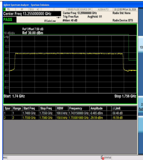
Band4-15MHz-16QAM-20325-1RB#74-PASS
