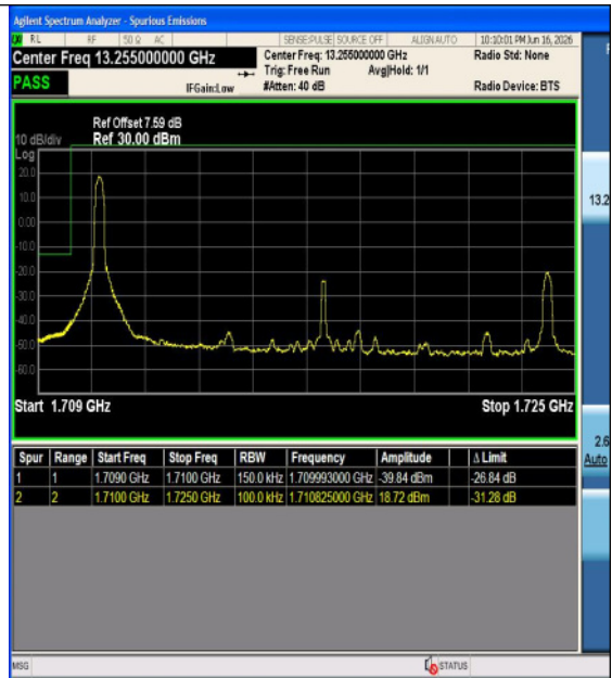
Band4-15MHz-QPSK-20325-1RB#0-PASS
