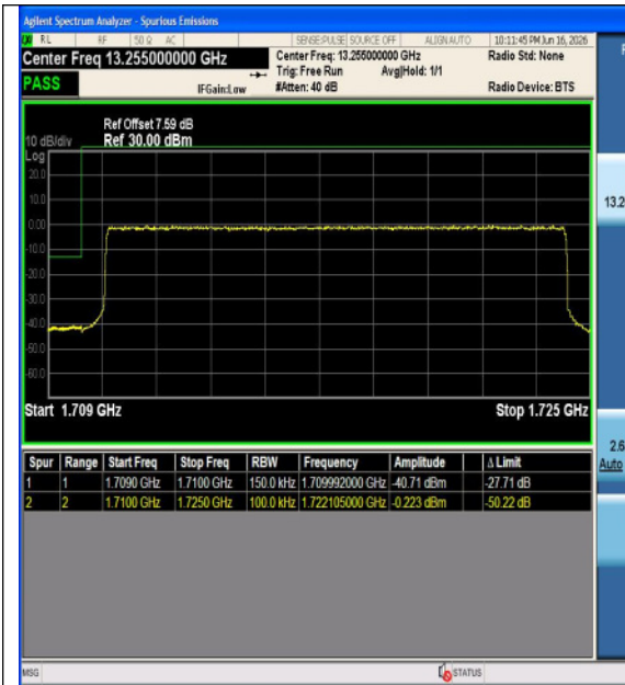
Band4-15MHz-16QAM-20025-1RB#74-PASS
