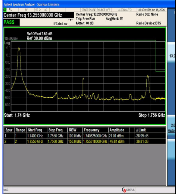
Band4-15MHz-QPSK-20325-75RB#0-PASS
