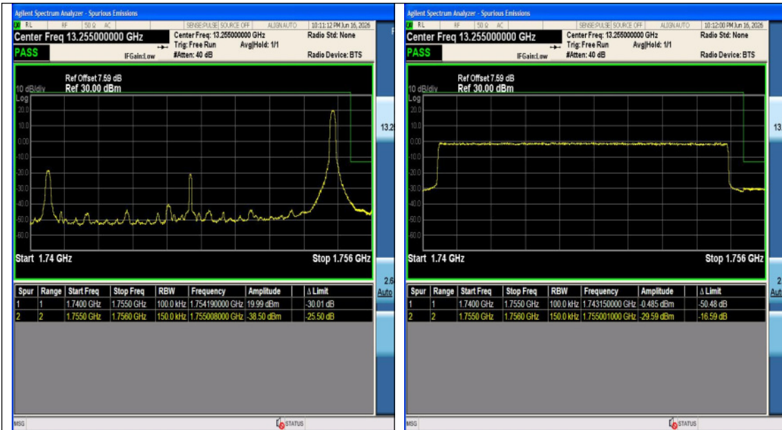
Band4-15MHz-16QAM-20325-1RB#0-PASS
