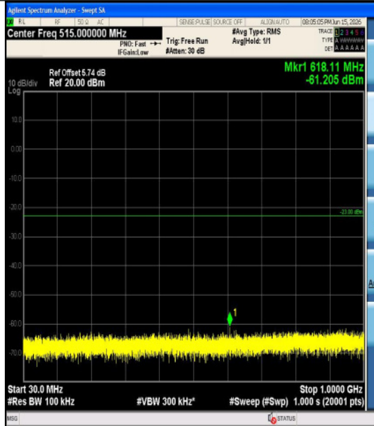
Band4-1.4MHz-16QAM-19957-6RB#0-3000~200 00-PASS
