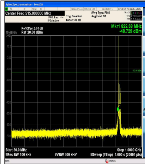
Band5-10MHz-QPSK-20450-1RB#0-3000~1000 0-PASS
