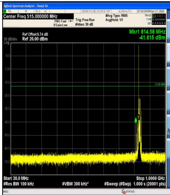
Band5-10MHz-QPSK-20525-1RB#0-3000~1000 0-PASS
