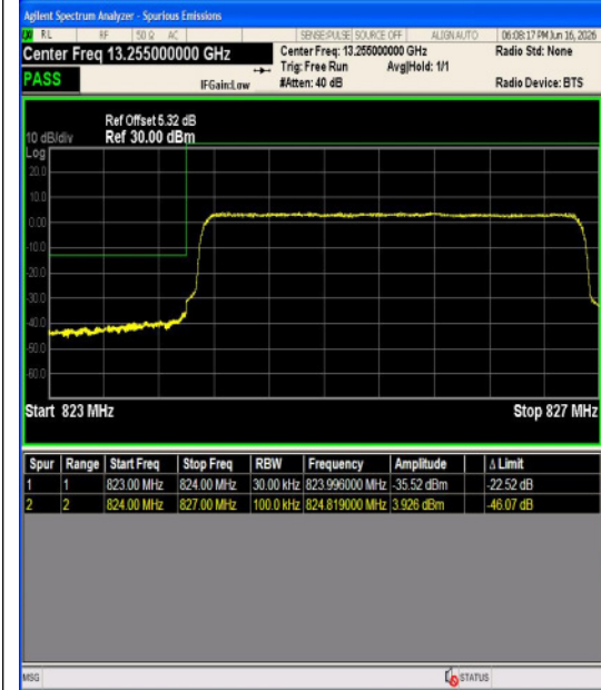
Band5-3MHz-16QAM-20415-1RB#14-PASS
