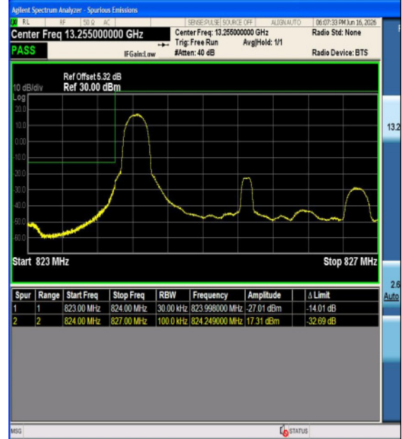
Band5-3MHz-16QAM-20415-15RB#0-PASS
