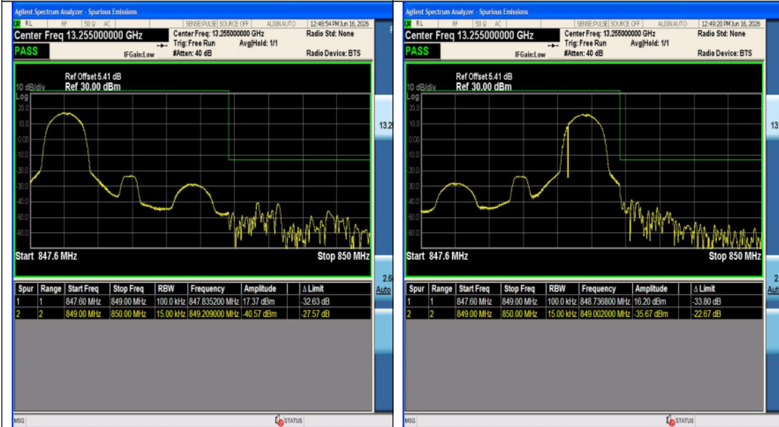
Band5-1.4MHz-QPSK-20643-6RB#0-PASS
