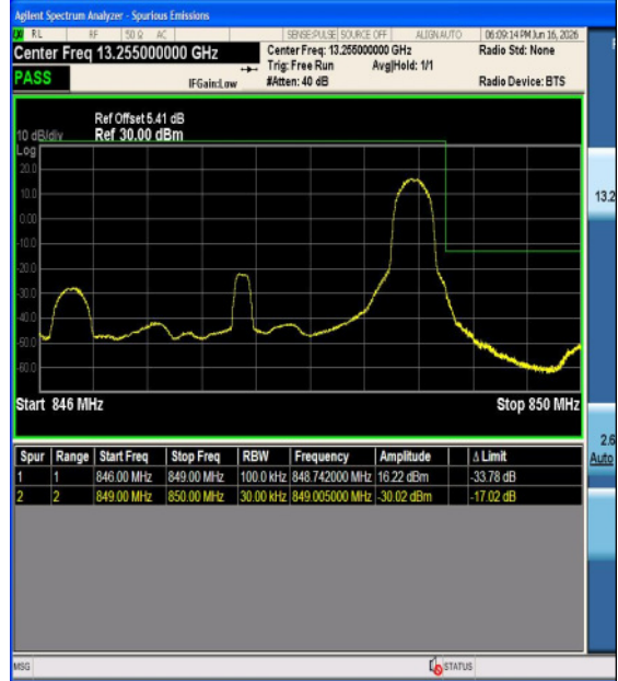
Band5-3MHz-16QAM-20635-1RB#0-PASS
