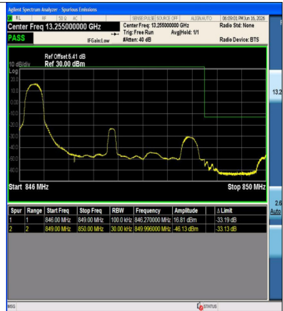
Band5-3MHz-16QAM-20635-15RB#0-PASS
