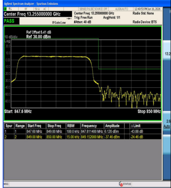
Band5-3MHz-QPSK-20415-1RB#14-PASS
