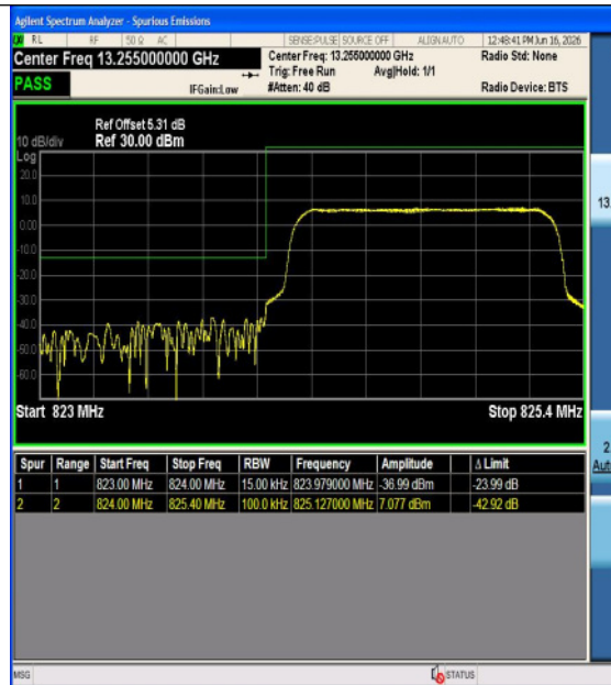
Band5-1.4MHz-QPSK-20643-1RB#5-PASS
