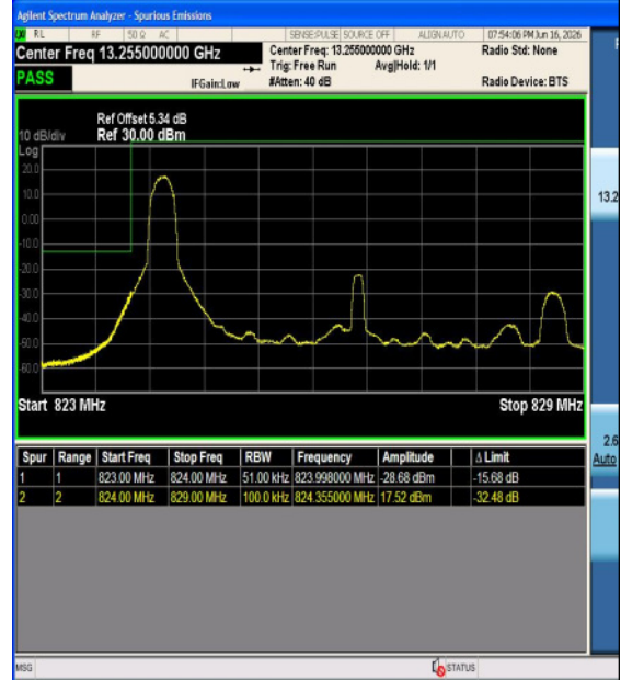
Band5-5MHz-16QAM-20425-25RB#0-PASS
