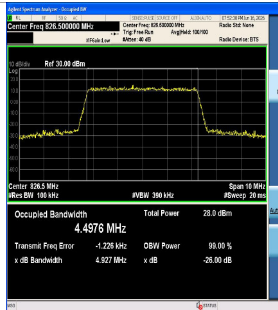
Band5-5MHz-16QAM-20525-25RB#0-PASS
