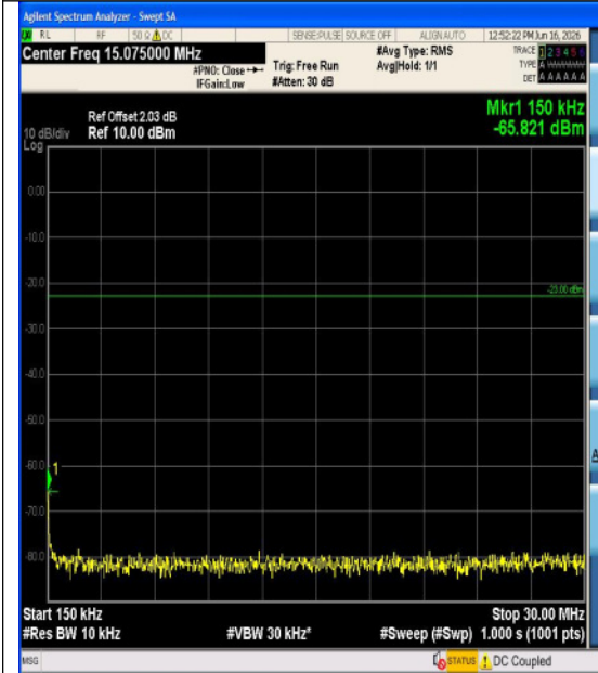
Band5-1.4MHz-QPSK-20407-1RB#5-1000~3000 -PASS
