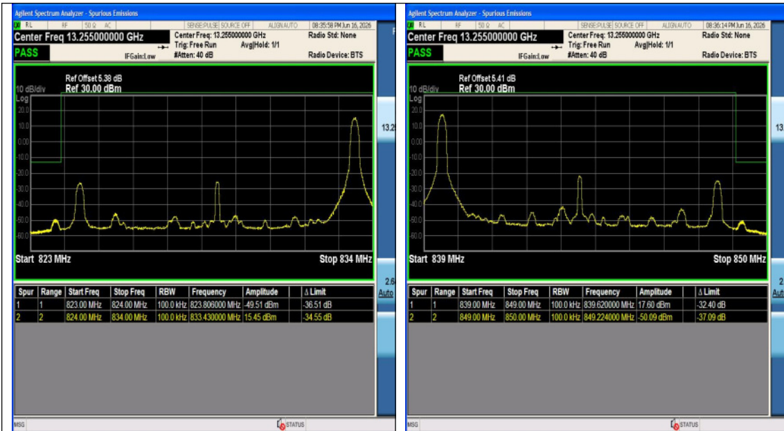
Band5-10MHz-QPSK-20600-1RB#49-PASS
