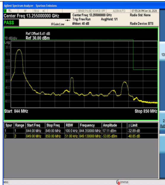
Band5-5MHz-16QAM-20625-25RB#0-PASS
