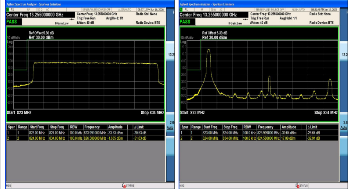
Band5-10MHz-16QAM-20450-1RB#49-PASS
