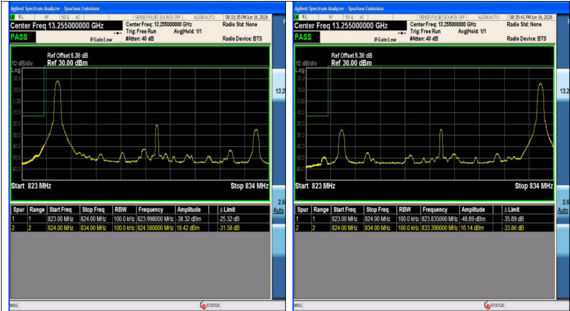
Band5-10MHz-QPSK-20450-50RB#0-PASS
