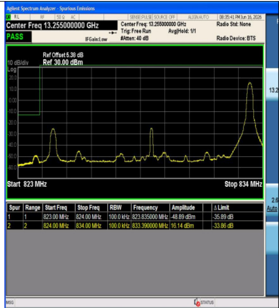
Band5-10MHz-16QAM-20450-1RB#0-PASS
