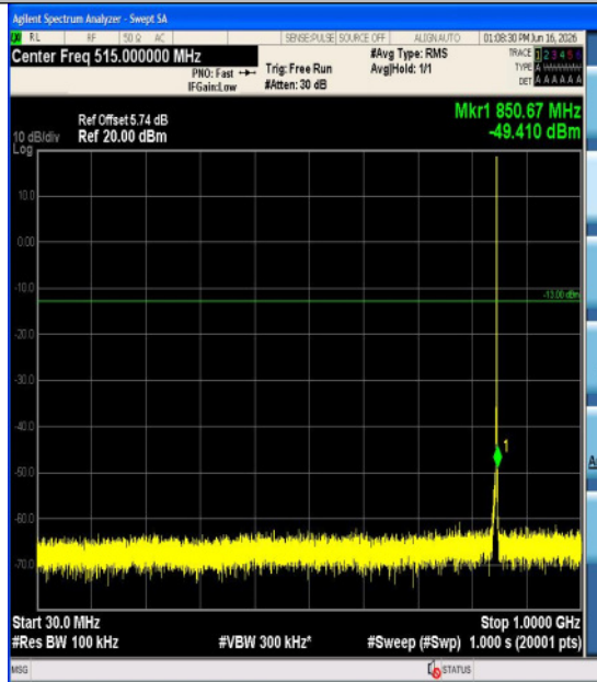
Band5-1.4MHz-QPSK-20643-1RB#5-3000~1000 0-PASS
