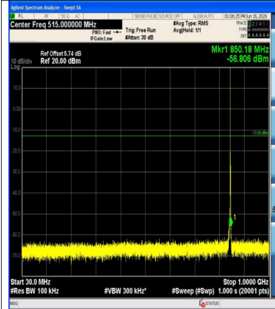
Band5-1.4MHz-QPSK-20643-1RB#0-3000~1000 0-PASS
