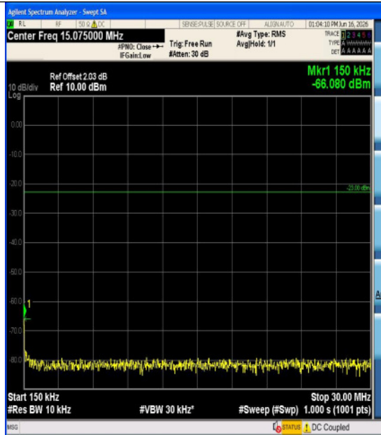
Band5-1.4MHz-QPSK-20525-6RB#0-1000~3000 -PASS
