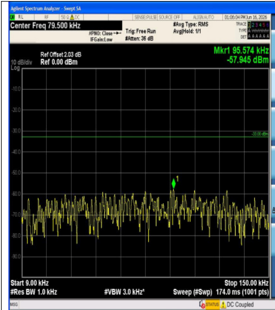
Band5-1.4MHz-QPSK-20643-1RB#0-30~1000-P ASS
