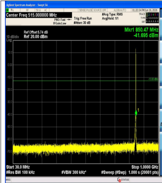
Band5-1.4MHz-QPSK-20643-6RB#0-3000~1000 0-PASS
