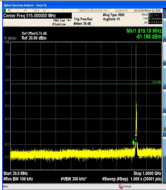
Band5-3MHz-16QAM-20525-1RB#0-3000~1000 0-PASS
