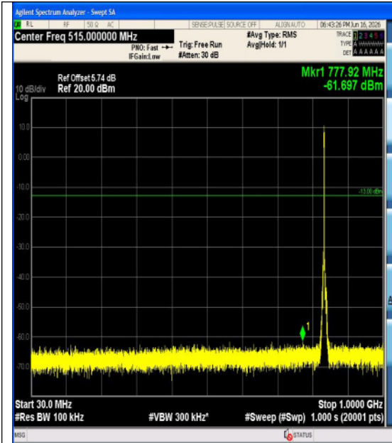
Band5-3MHz-QPSK-20525-15RB#0-3000~1000 0-PASS
