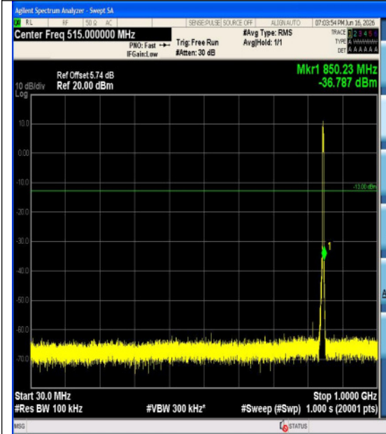
Band5-3MHz-QPSK-20635-15RB#0-3000~1000 0-PASS
