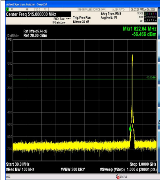
Band5-5MHz-QPSK-20525-25RB#0-3000~1000 0-PASS
