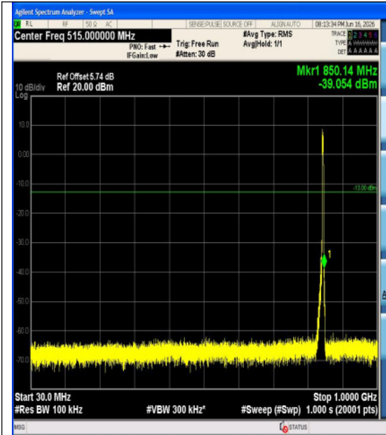
Band5-5MHz-QPSK-20625-25RB#0-3000~1000 0-PASS
