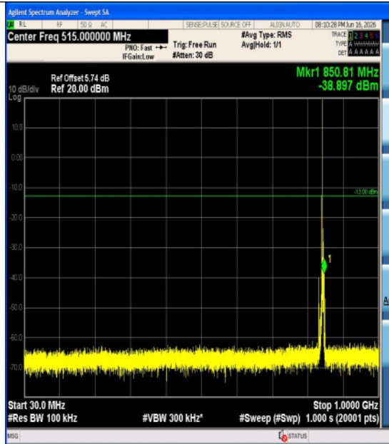
Band5-5MHz-16QAM-20625-1RB#0-3000~1000 0-PASS
