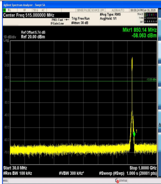
Band5-5MHz-16QAM-20525-25RB#0-3000~100 00-PASS
