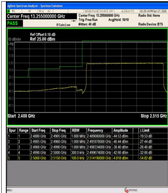
Band7-15MHz-16QAM-20825-1RB#74-PASS
