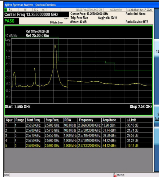
Band7-5MHz-16QAM-21425-1RB#0-PASS
