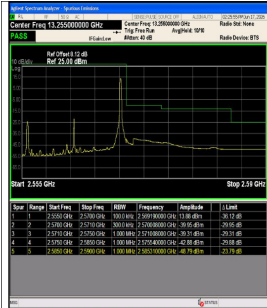
Band7-15MHz-16QAM-21375-1RB#0-PASS
