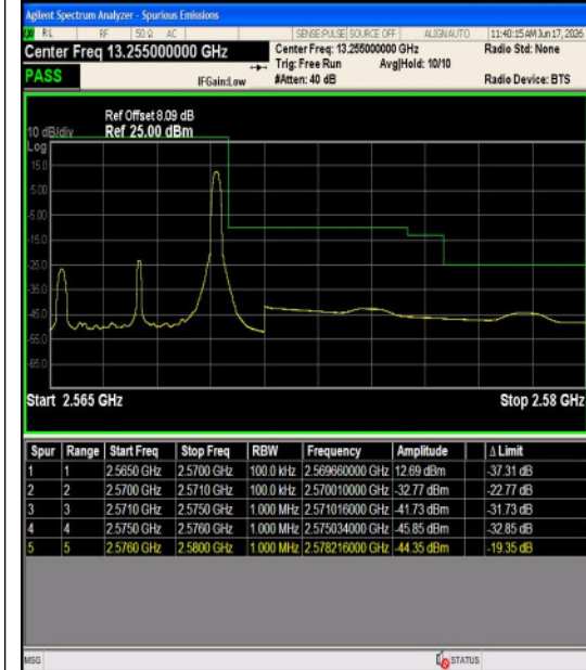
Band7-10MHz-QPSK-20800-1RB#0-PASS
