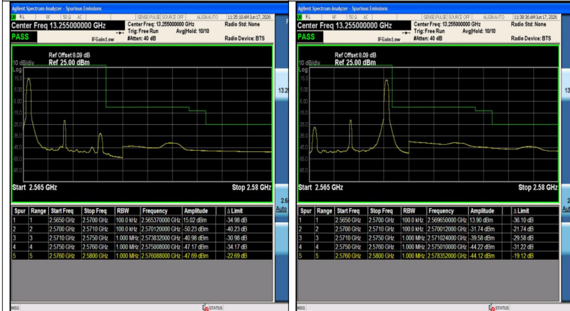
Band7-5MHz-QPSK-21425-25RB#0-PASS
