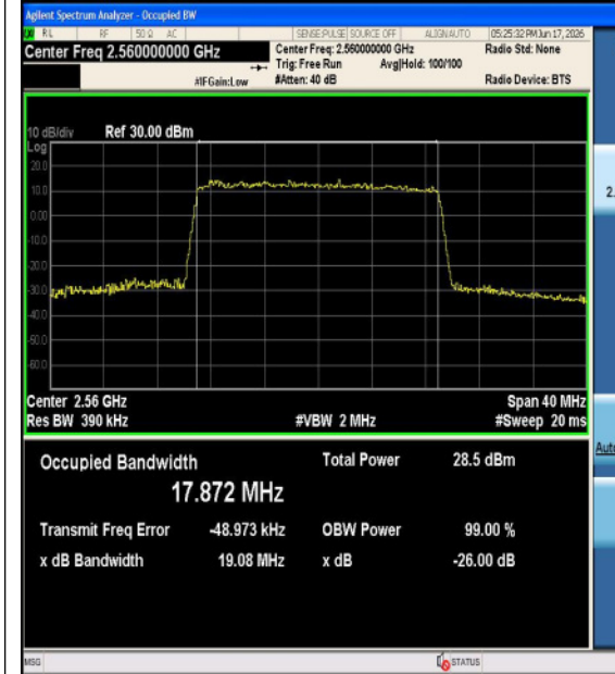
Band7-20MHz-QPSK-21350-100RB#0-PASS
