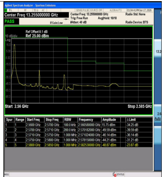
Band7-10MHz-QPSK-21400-50RB#0-PASS
