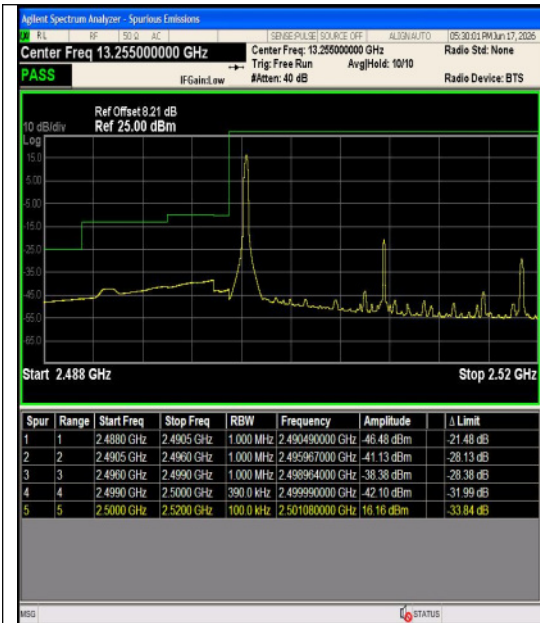
Band7-20MHz-QPSK-20850-100RB#0-PASS
