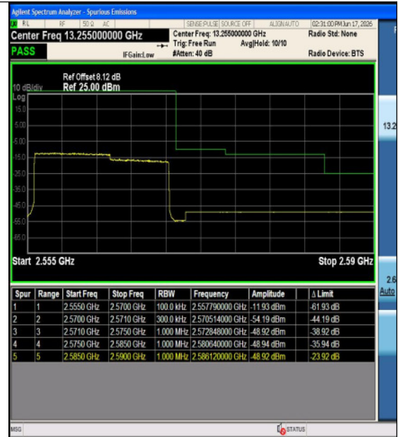
Band7-15MHz-16QAM-21375-1RB#74-PASS
