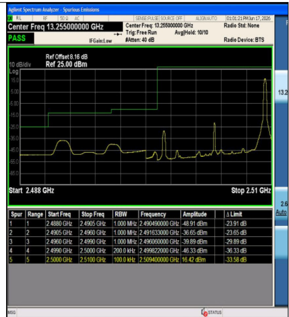
Band7-10MHz-16QAM-20800-1RB#0-PASS
