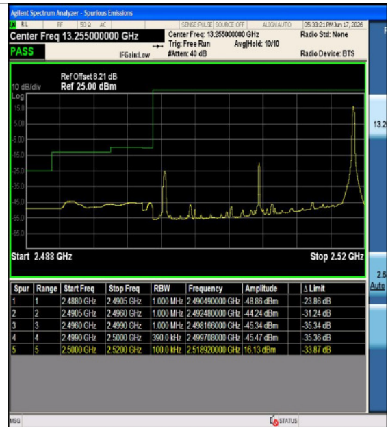
Band7-20MHz-16QAM-20850-1RB#0-PASS
