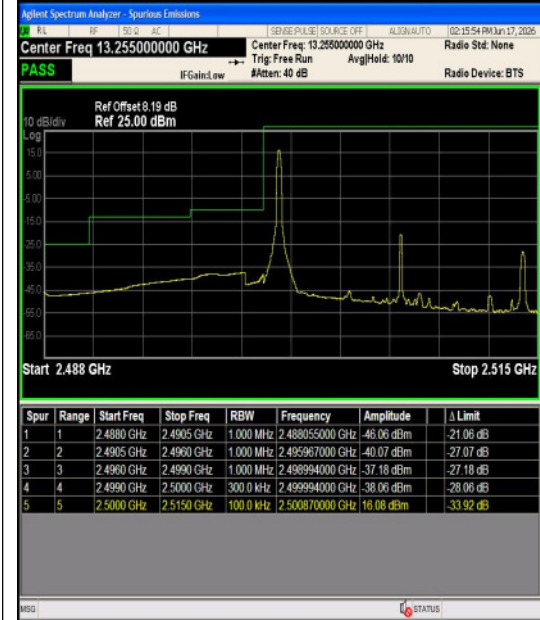
Band7-15MHz-QPSK-20825-75RB#0-PASS
