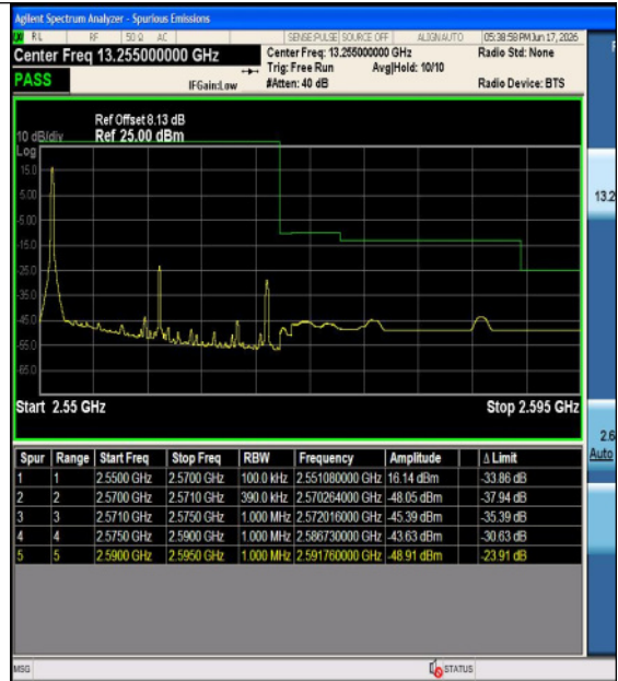
Band7-20MHz-QPSK-21350-100RB#0-PASS
