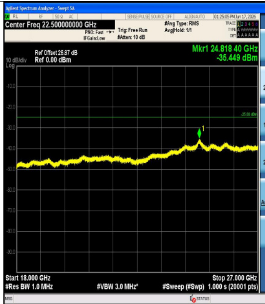
Band7-10MHz-QPSK-21100-50RB#0-0.15~30-P ASS
