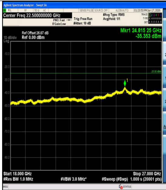
Band7-10MHz-16QAM-21100-1RB#49-0.15~30- PASS
