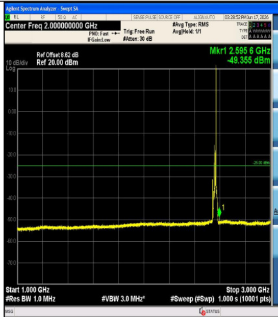
Band7-15MHz-QPSK-21375-1RB#74-18000~27 000-PASS
