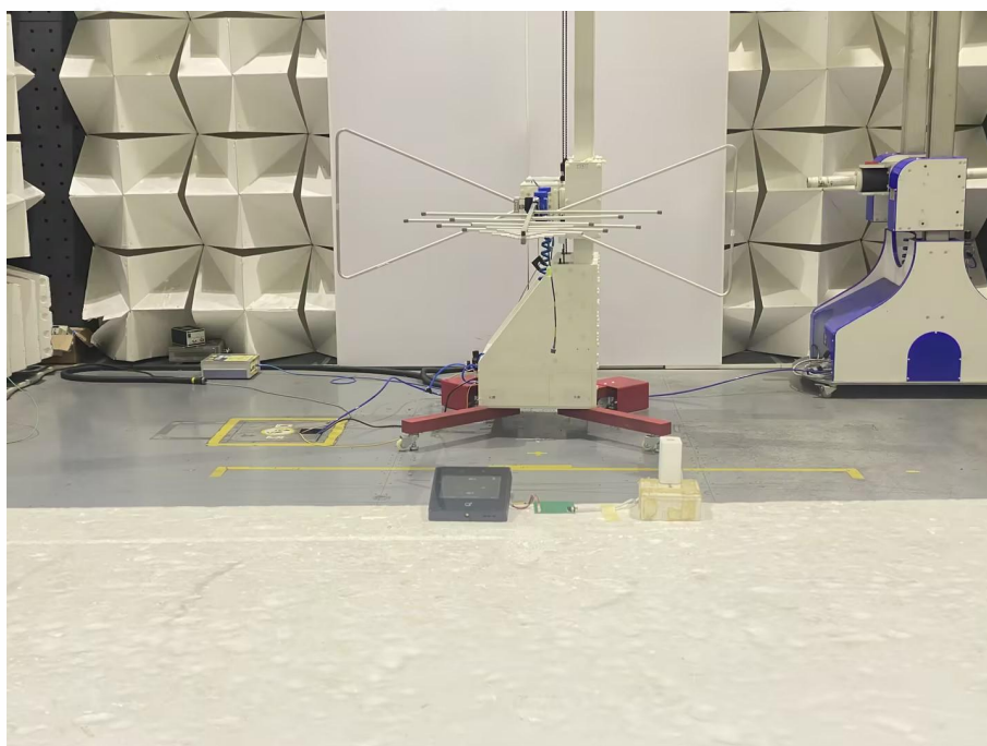
Radiated spurious emission Test Setup-2 close up(Below 1GHz)
