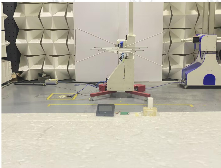
Radiated Spurious Emissions Test Setup (30MHz~1GHz) close up
