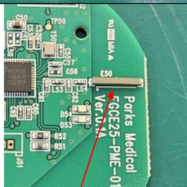
Chip Antenna
