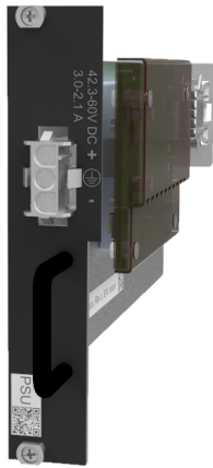
PSU1 (Left Slot orientation)
