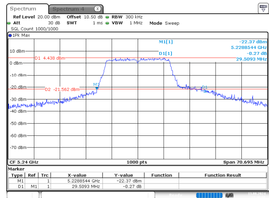
n20_5240MHz
