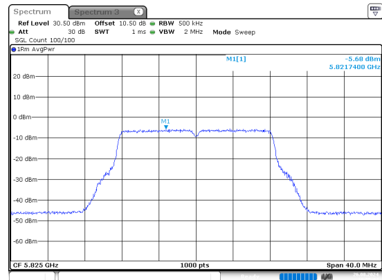
a_5825MHz
