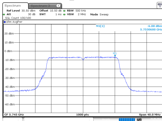
n20_5745MHz
