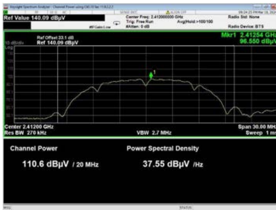
Figure 7 – Radiated Output Power Field Strength, WiFi B, Low Data Rate, Low Channel.
