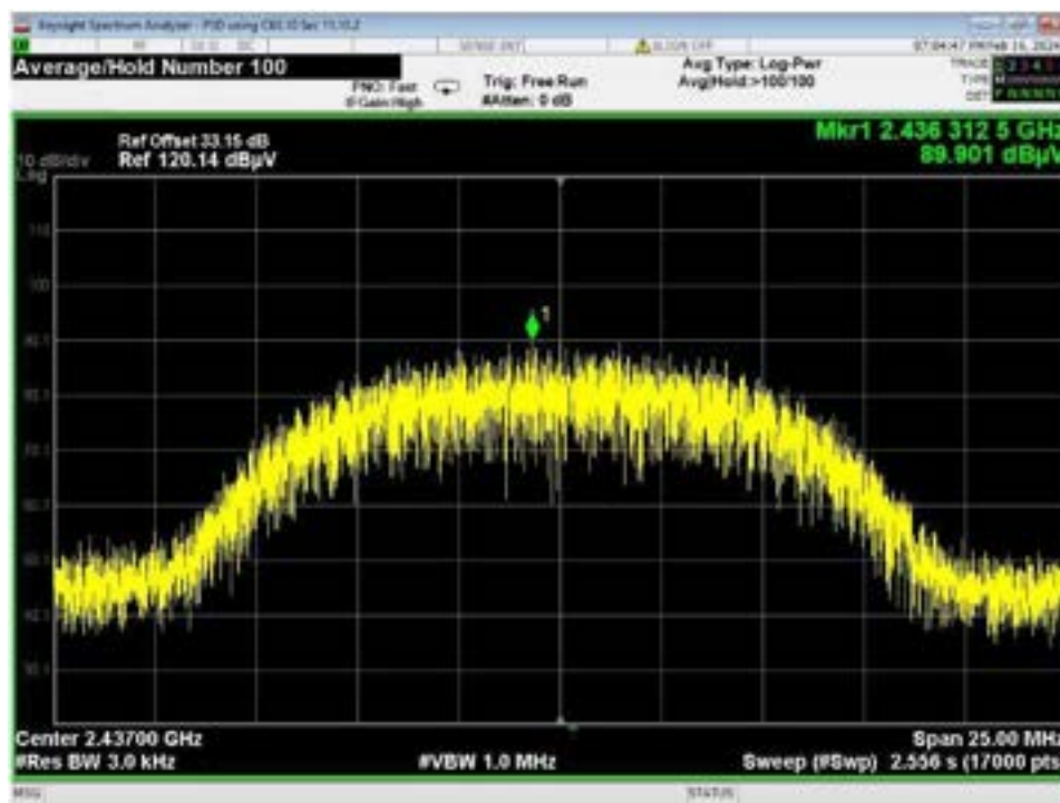
Figure 72 – Radiated EIRP Power Spectral Density, WiFi B, High Data Rate, Mid Channel
