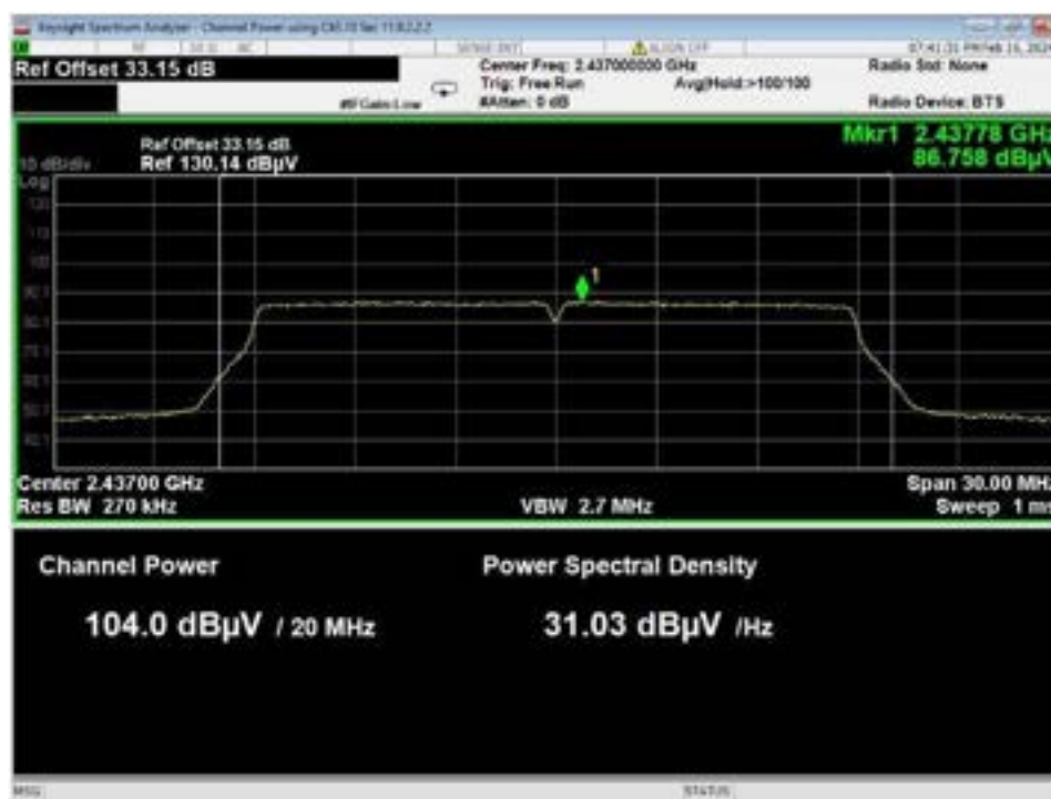
Figure 20 – Radiated Output Power Field Strength, WiFi N, Low Data Rate, Mid Channel
