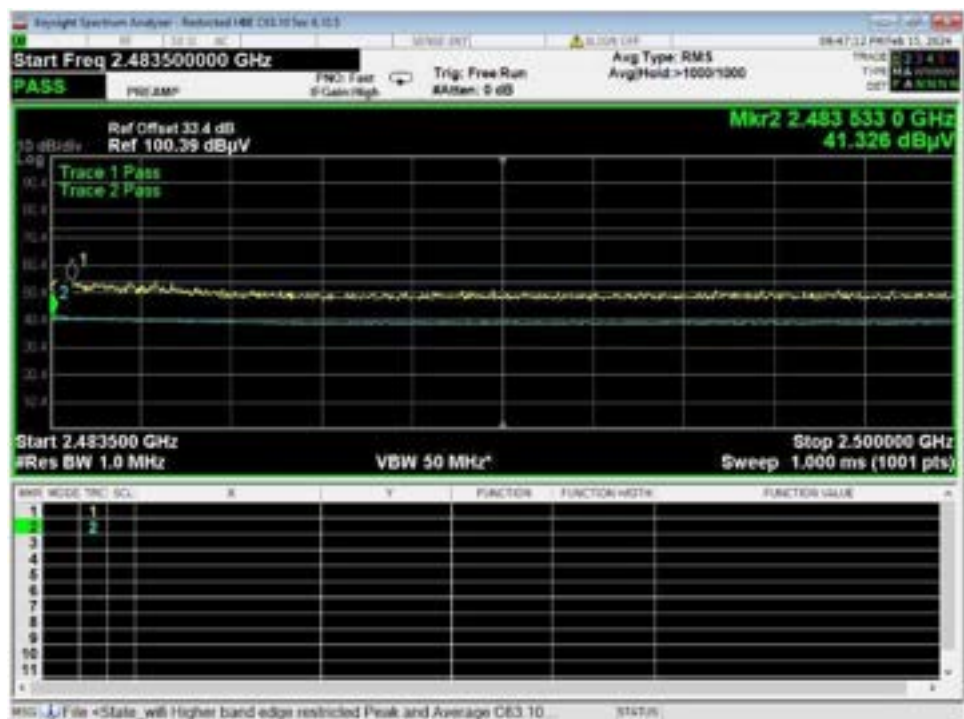
Figure 53 – Band-edge Measurement, WiFi N, Low Data Rate, High Channel, Restricted Frequency
