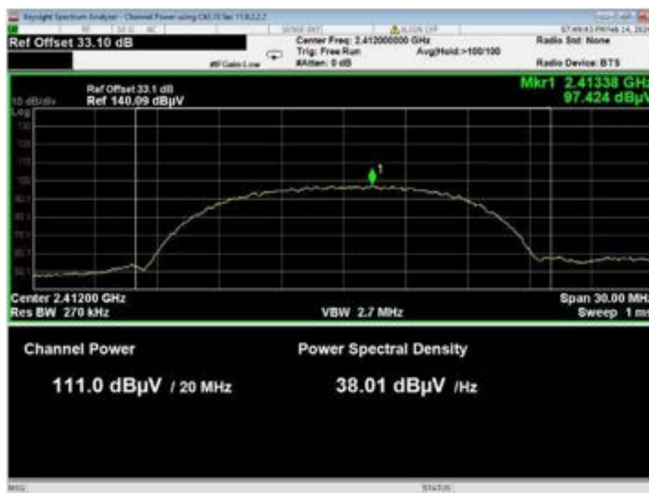
Figure 10 – Radiated Output Power Field Strength, WiFi B, High Data Rate, Low Channel.
