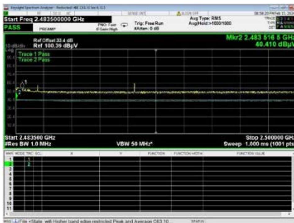
Figure 49 – Band-edge Measurement, WiFi G, Low Data Rate, High Channel, Restricted Frequency
