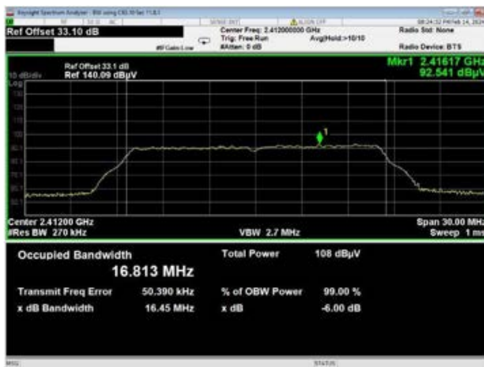
Figure 32 –Bandwidth, WiFi G, Low Data Rate, Low Channel
