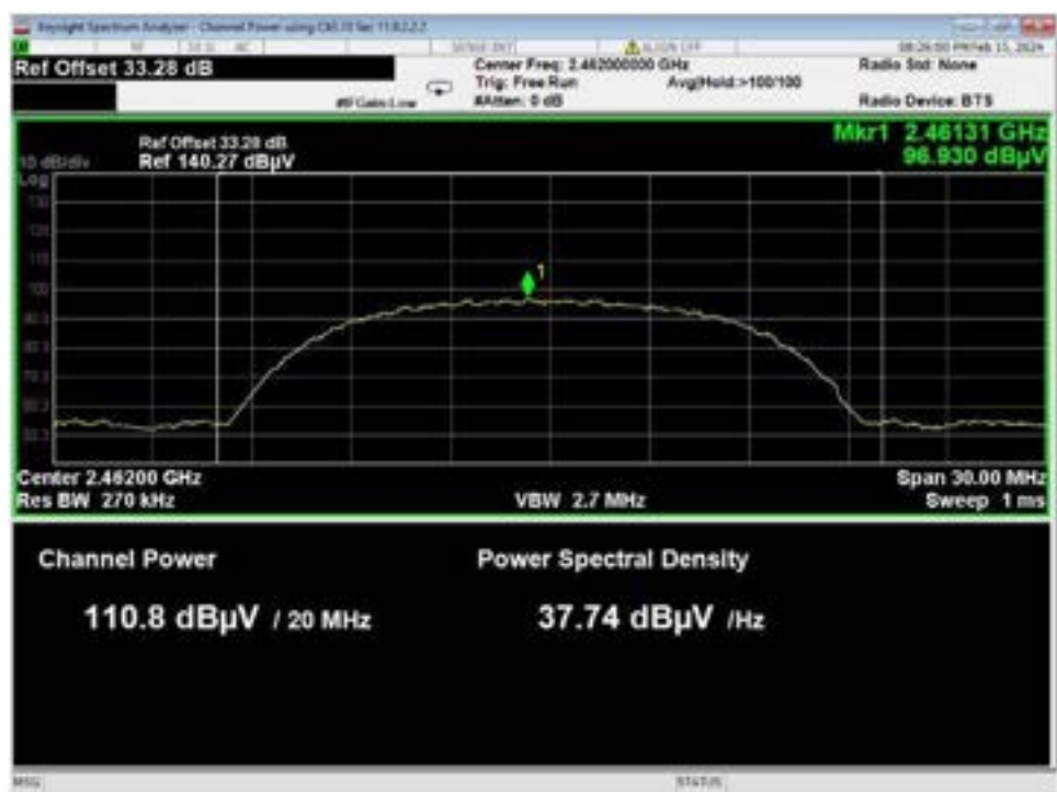
Figure 12 – Radiated Output Power Field Strength, WiFi B, High Data Rate, High Channel
