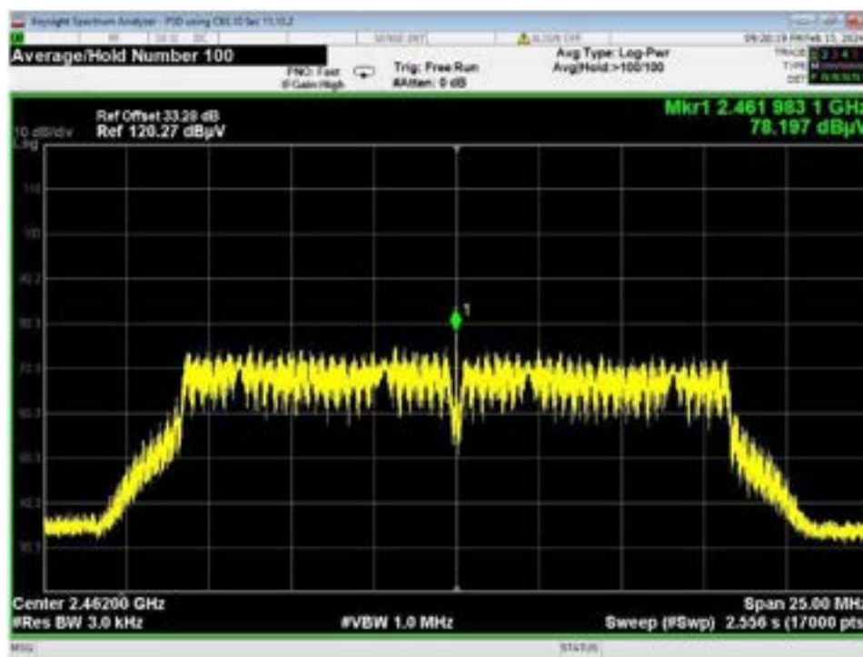
Figure 79 – Radiated EIRP Power Spectral Density, WiFi G, High Data Rate, High Channel
