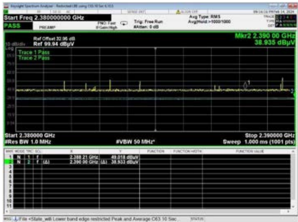
Figure 52 – Band-edge Measurement, WiFi N, Low Data Rate, Low Channel, Restricted Frequency
