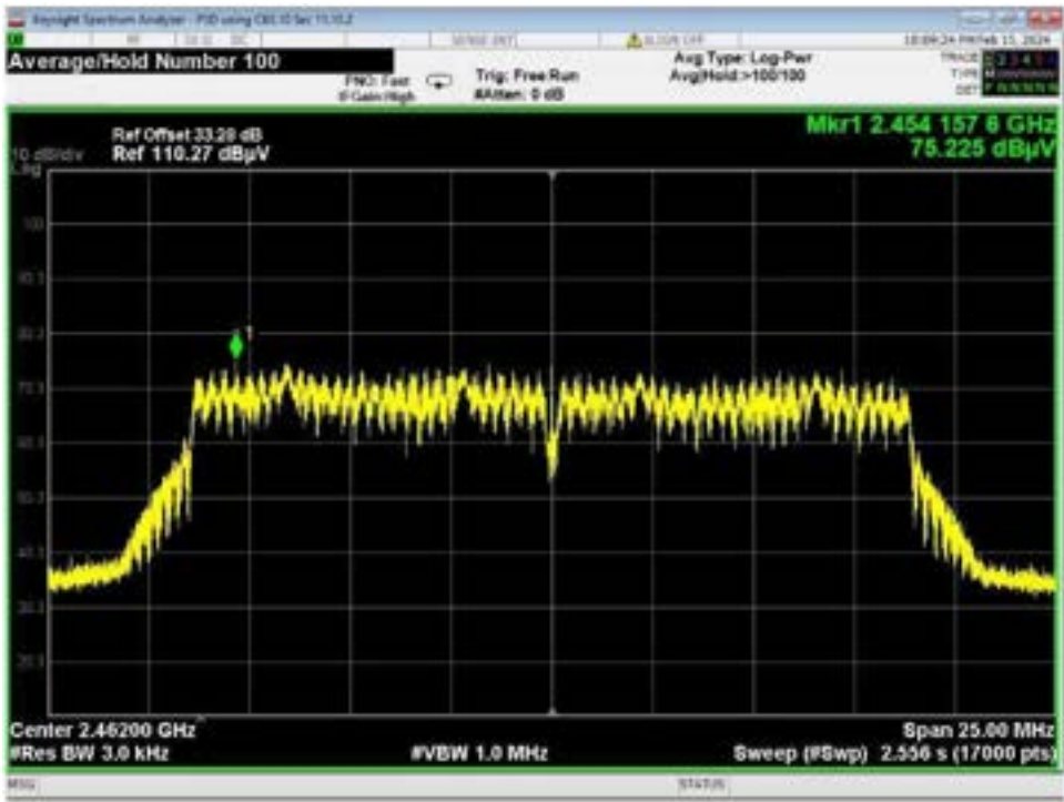
Figure 85 – Radiated EIRP Power Spectral Density, WiFi N, High Data Rate, High Channel
