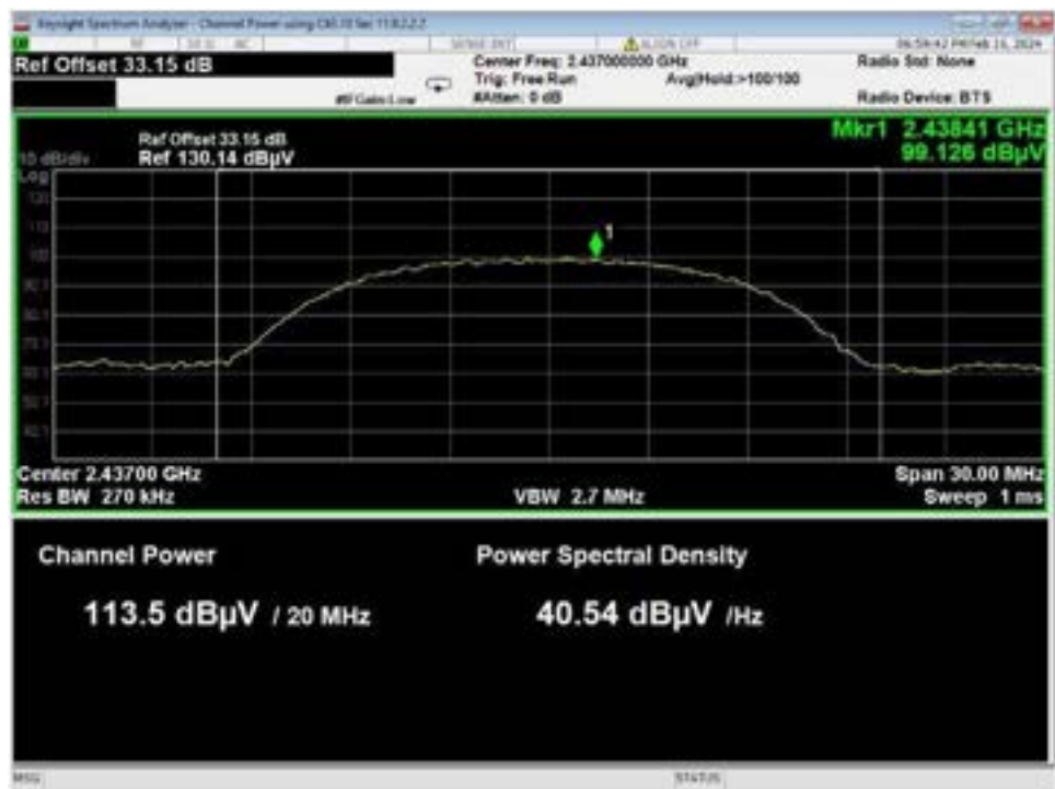
Figure 11 – Radiated Output Power Field Strength, WiFi B, High Data Rate, Mid Channel
