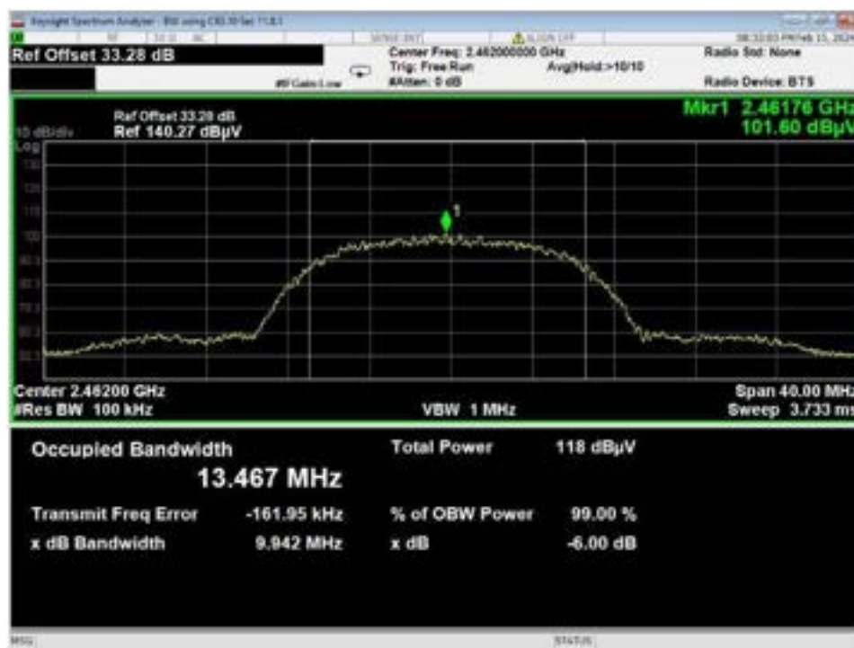
Figure 31 - Bandwidth, WiFi B, High Data Rate, High Channel
