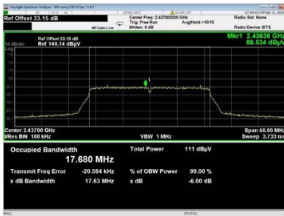
Figure 39 - Bandwidth, WiFi N, Low Data Rate, Mid Channel
