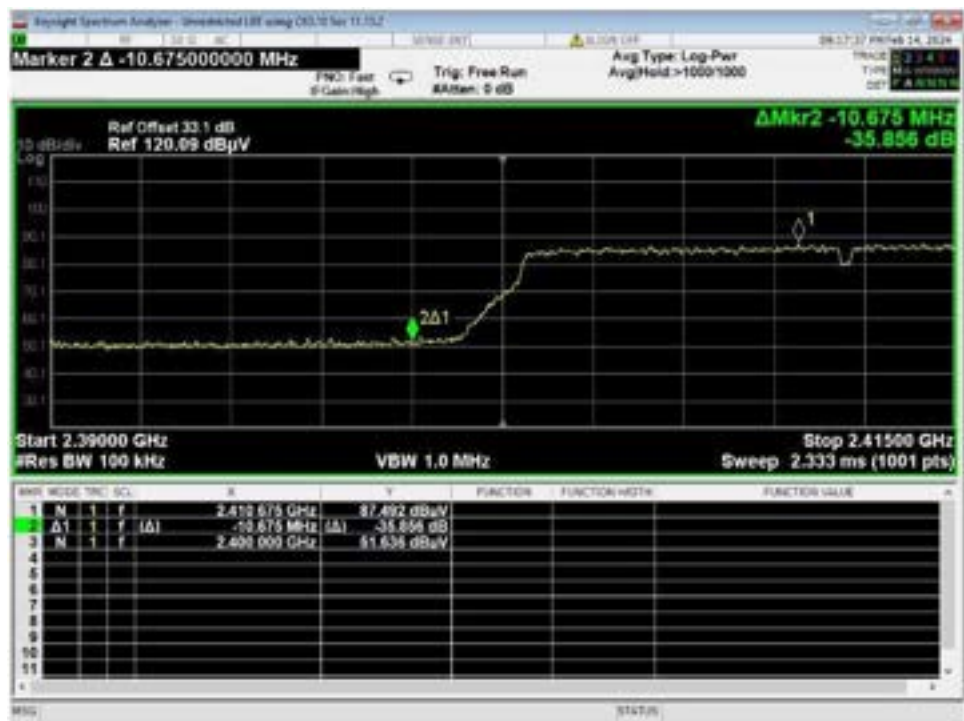
Figure 64 – Band-edge Measurement, WiFi N, Low Data Rate, Low Channel, Unrestricted Frequency
