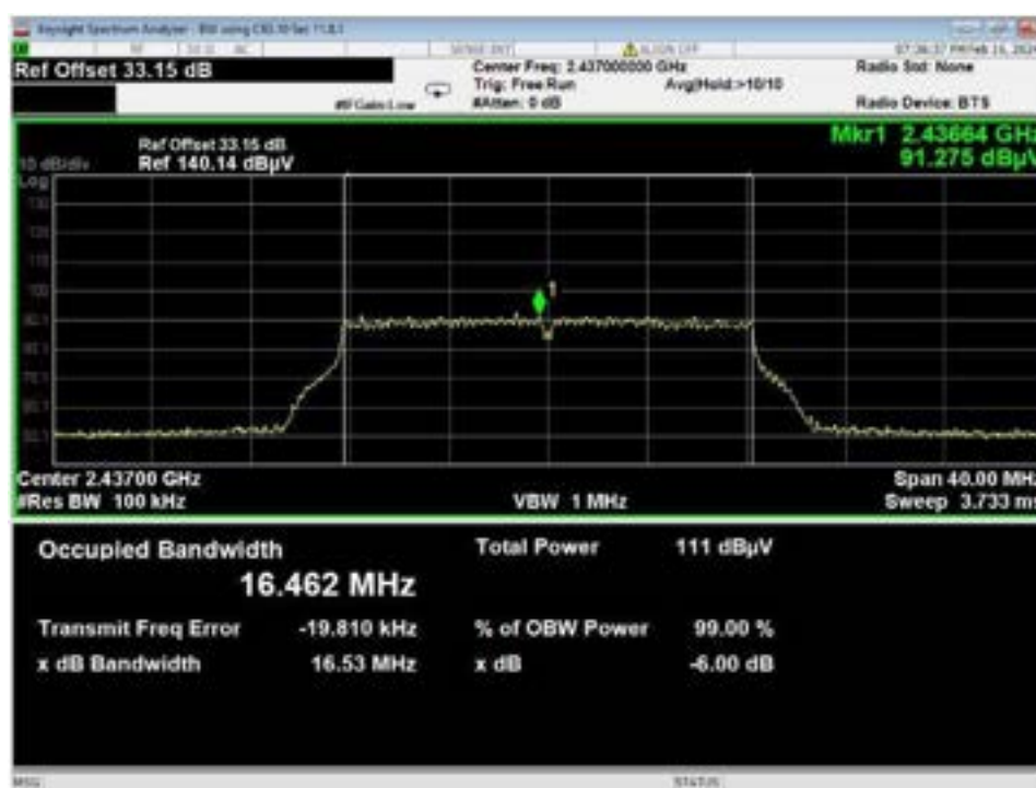
Figure 36 - Bandwidth, WiFi G, High Data Rate, Mid Channel
