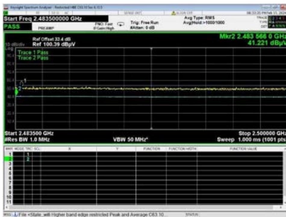
Figure 47 – Band-edge Measurement, WiFi B, High Data Rate, High Channel, Restricted Frequency
