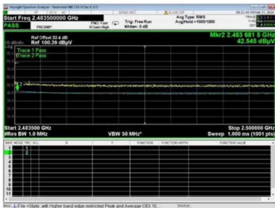
Figure 51 – Band-edge Measurement, WiFi G, High Data Rate, High Channel, Restricted Frequency
