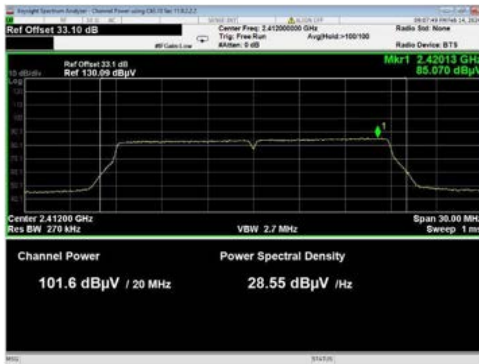
Figure 19 – Radiated Output Power Field Strength, WiFi N, Low Data Rate, Low Channel.
