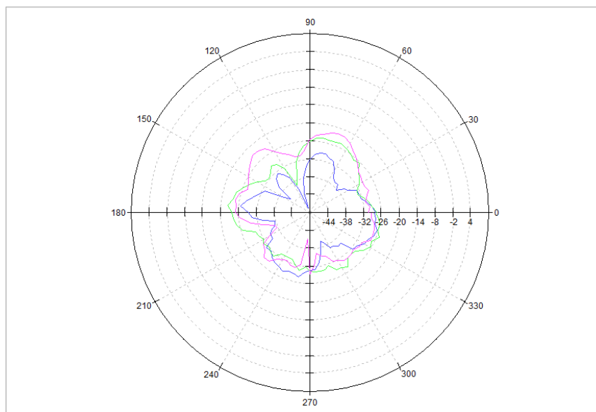
Figure 7.1-2: 2D antenna pattern, vertical polarization
