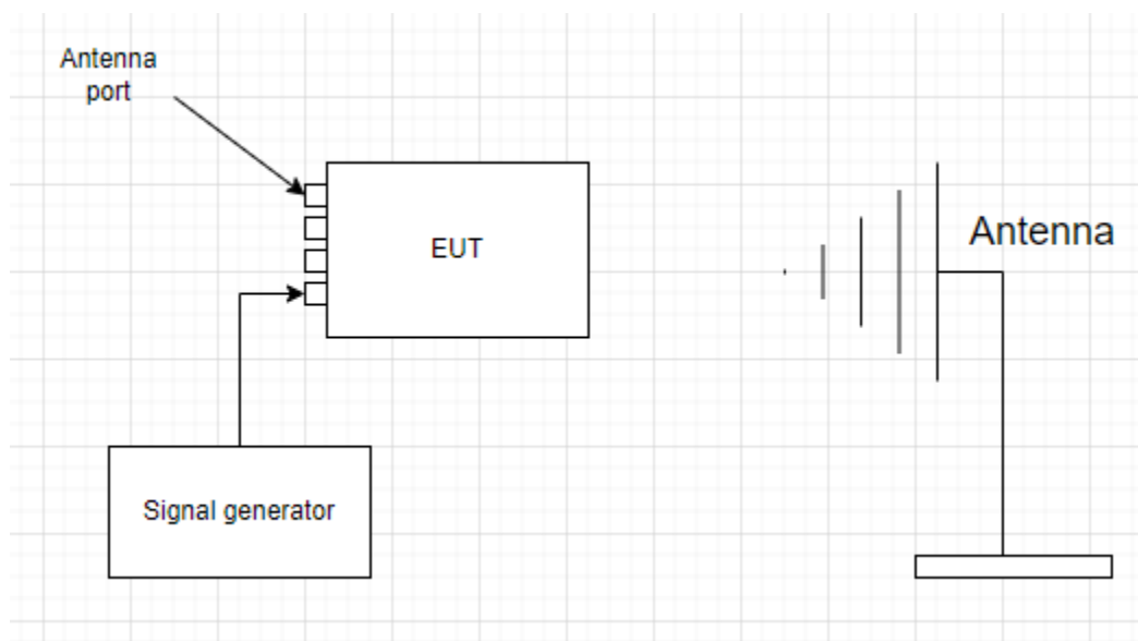
Figure 3.6-1: Test setup diagram
