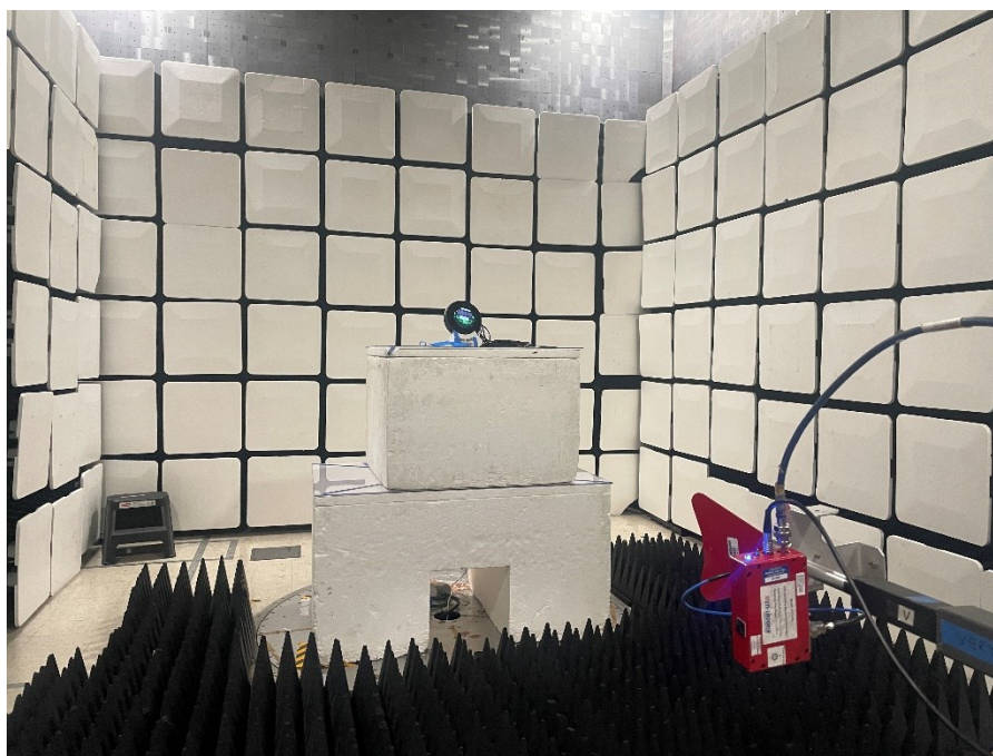
Figure 3 - Radiated emissions above 1 GHz (1 – 18 GHz), front view.
