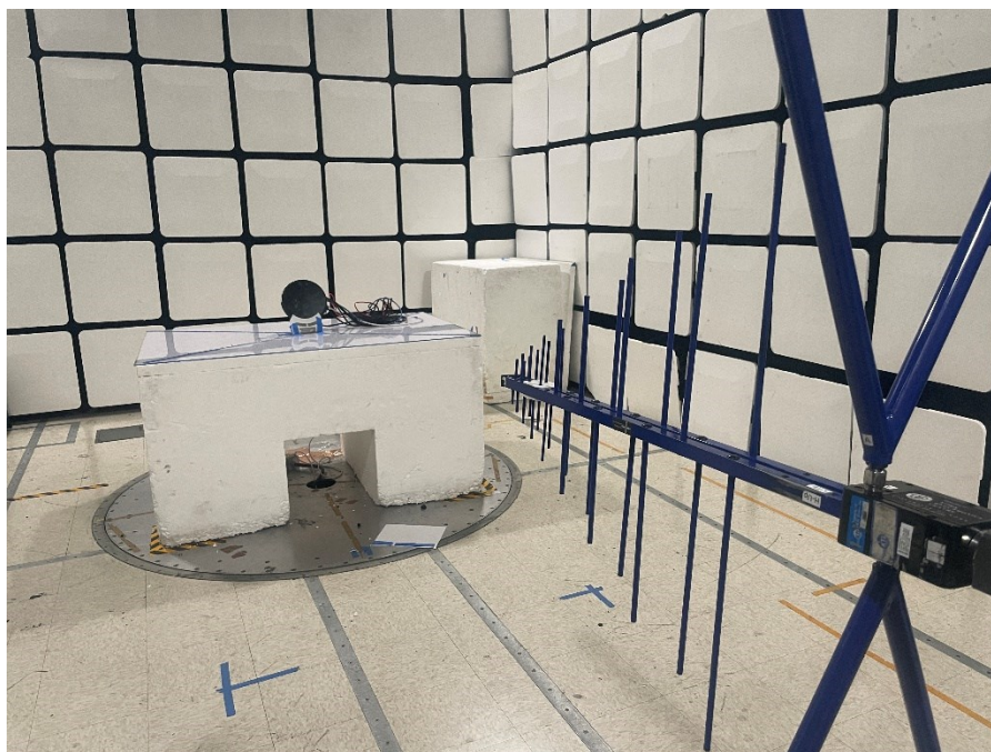
Figure 1 - Radiated emissions below 1 GHz (0.03 – 1 GHz), front view.
