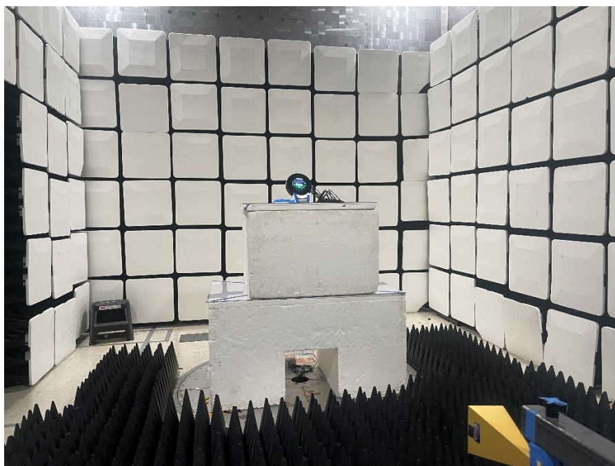
Figure 5 - Radiated emissions above 1 GHz (18 – 26 GHz), front view.
