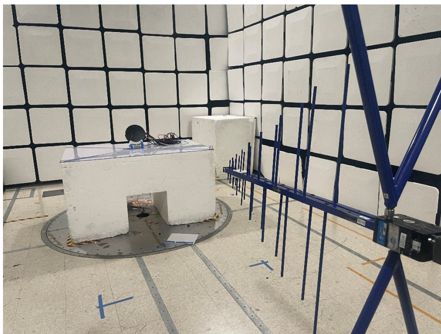
Figure 5 - Radiated emissions below 1 GHz (0.03 – 1 GHz), front view.
