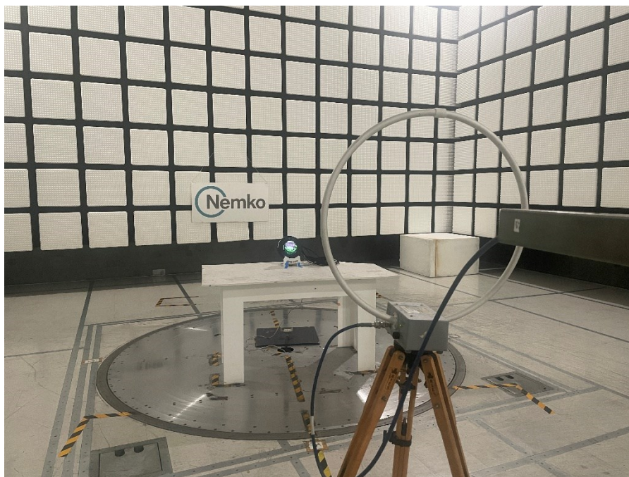
Figure 1 - Radiated emissions below 1 GHz (9k-30MHz), front view. 0 degree
