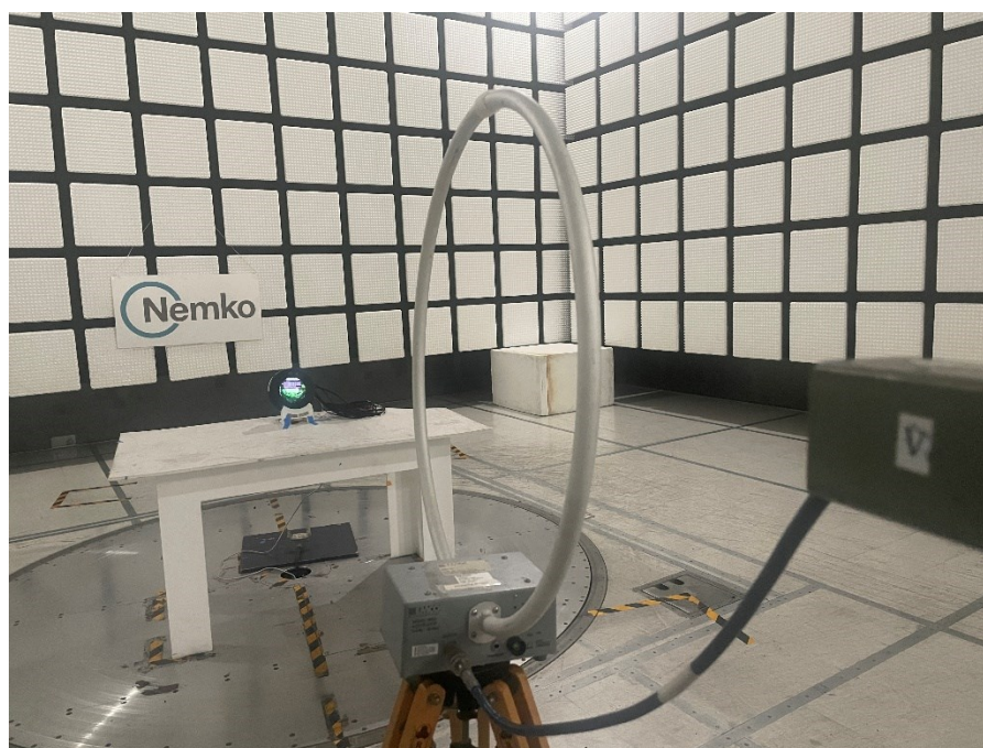
Figure 3 - Radiated emissions below 1 GHz (9k-30MHz), front view.90 degree
