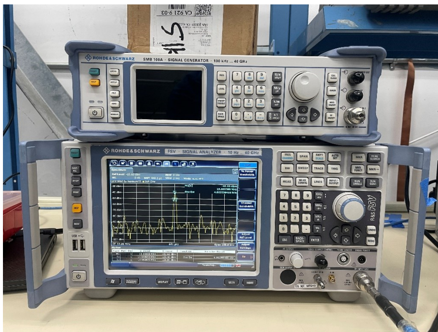
Figure 7 – Test setup (spectrum analyzer measurements)
