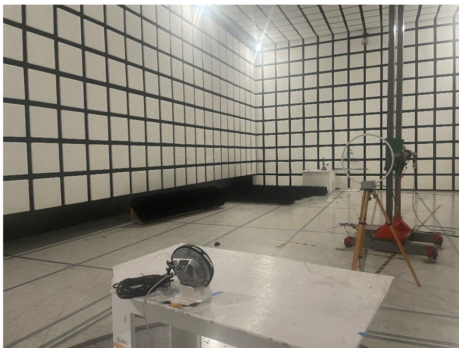
Figure 2 - Radiated emissions below 1 GHz (9k-30MHz), rear view. 0 degree
