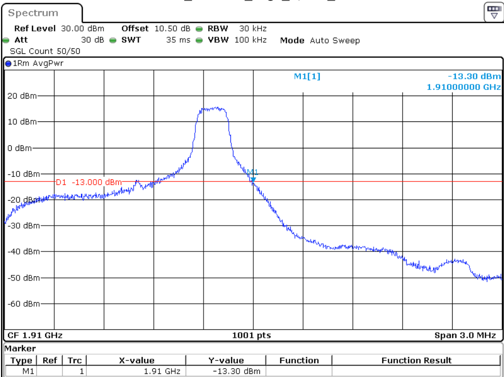
Band 2_1.4 MHz_High_QPSK_1RB
