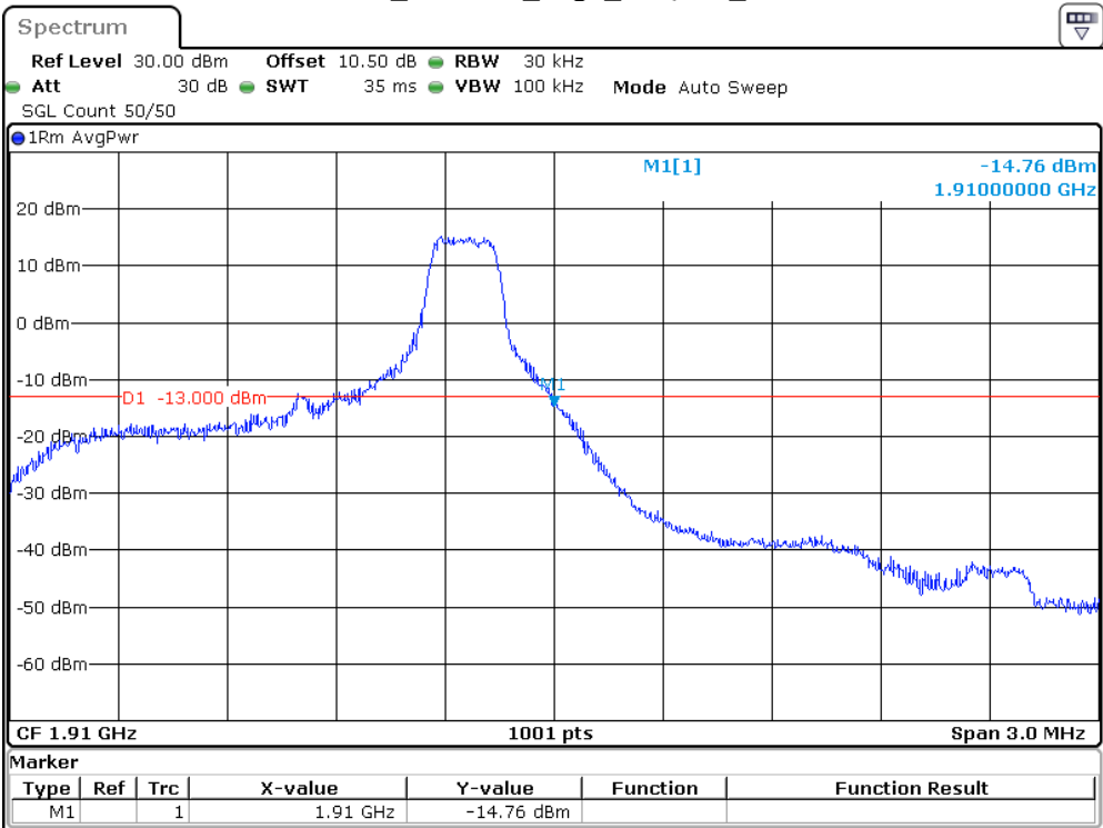
Band 2_1.4 MHz_High_16QAM_1RB
