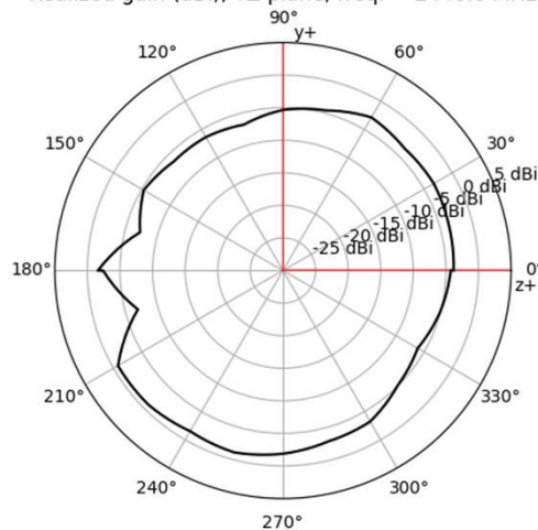
Realized gain (dBi), YZ-plane, freq. = 2440.0 MHz
