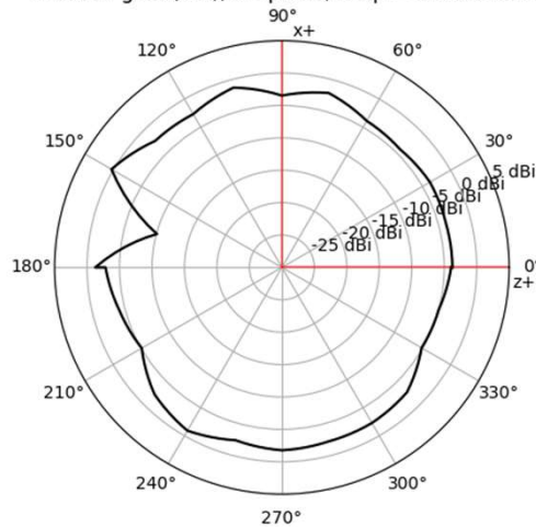
Realized gain (dBi), XZ-plane, freq. = 2440.0 MHz
