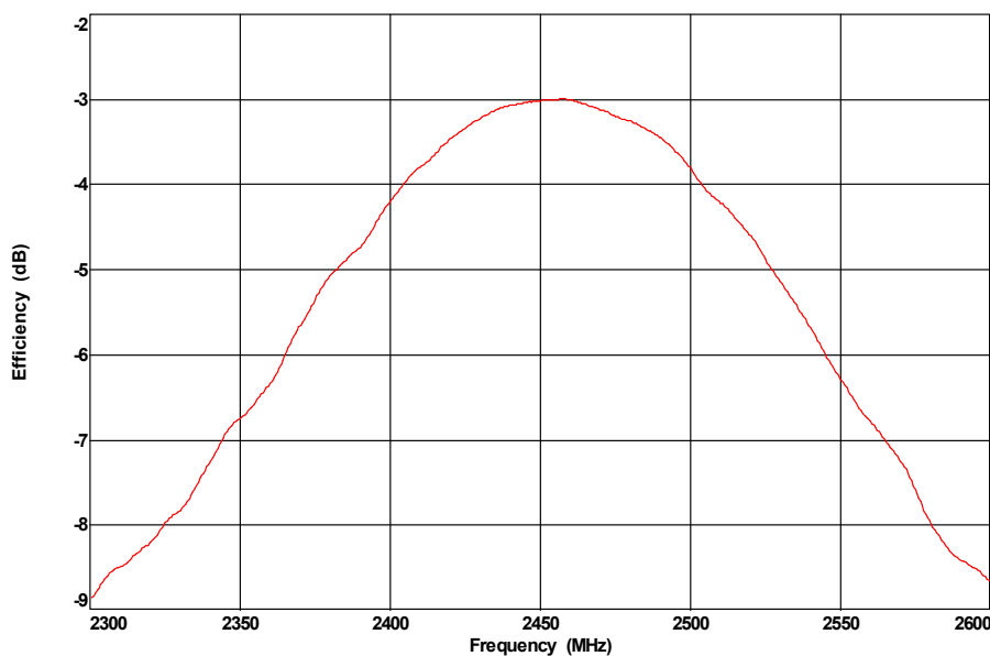
Total Antenna Efficiency
