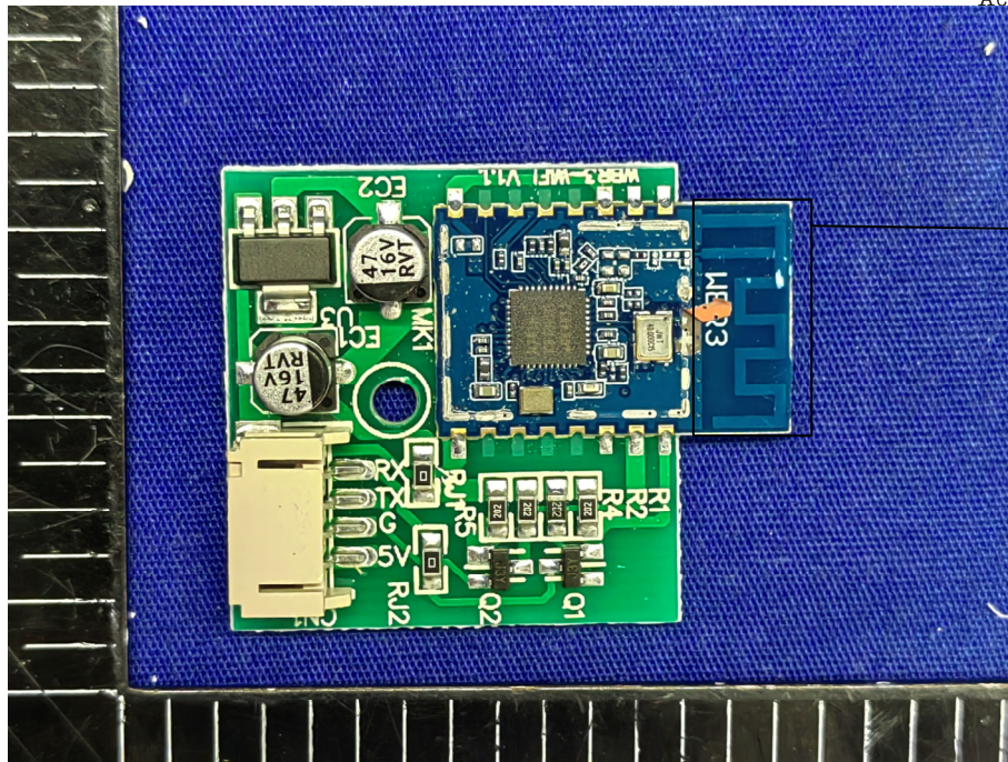
PCB antenna
