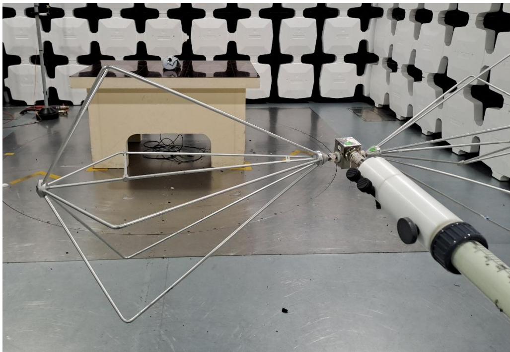
Photo 1 Photograph test setup radiated emissions 30-250 MHz, report section 3.1
