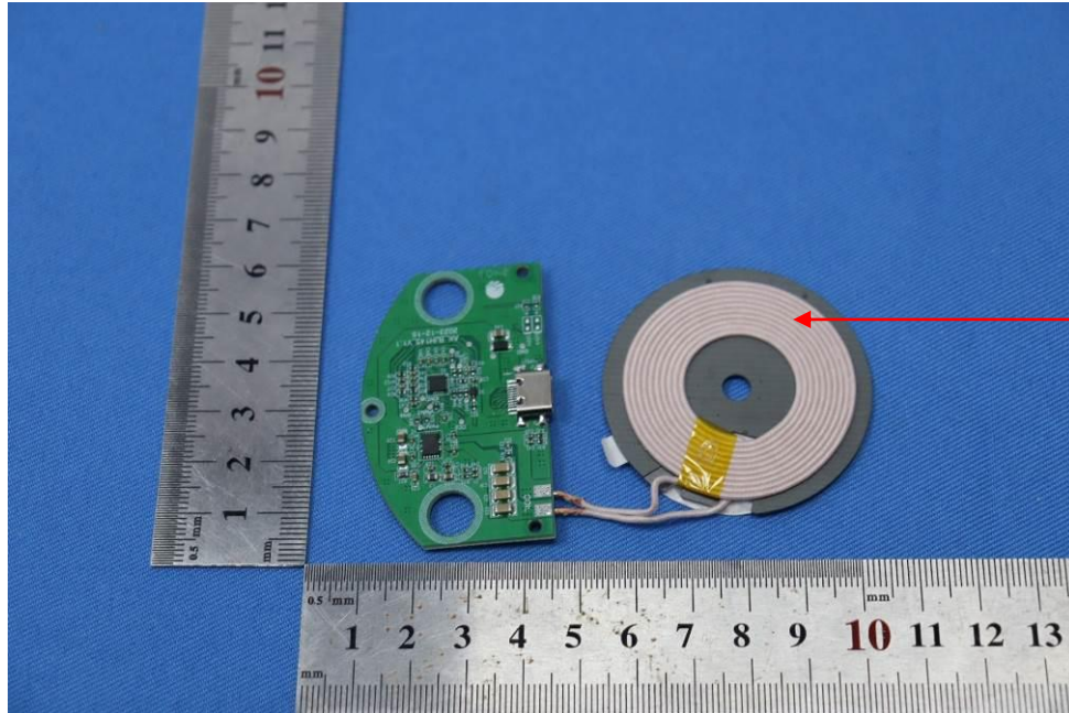
WPC antenna
