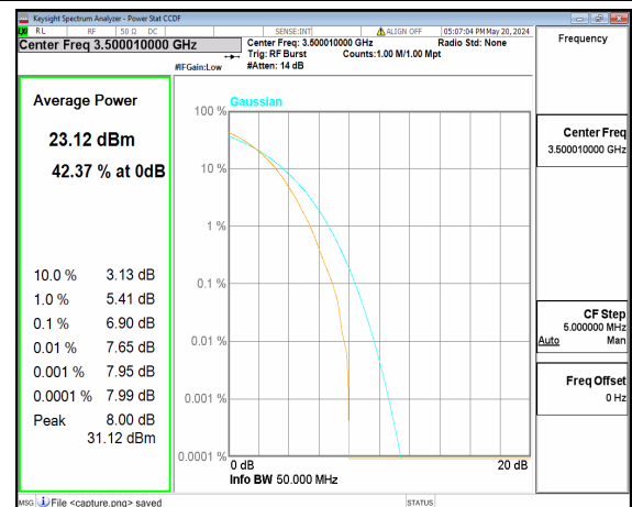
n77(3450-3550MHz) 50M DFT-s-OFDM 256QAM Outer_Full Mid
