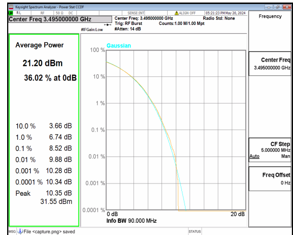
n77(3450-3550MHz) 90M CP-OFDM 256QAM Outer_Full Low
