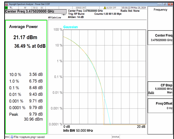
n77(3450-3550MHz) 50M CP-OFDM 256QAM Outer_Full Low
