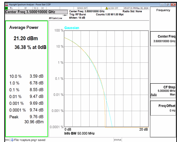
n77(3450-3550MHz) 50M CP-OFDM 256QAM Outer_Full Mid
