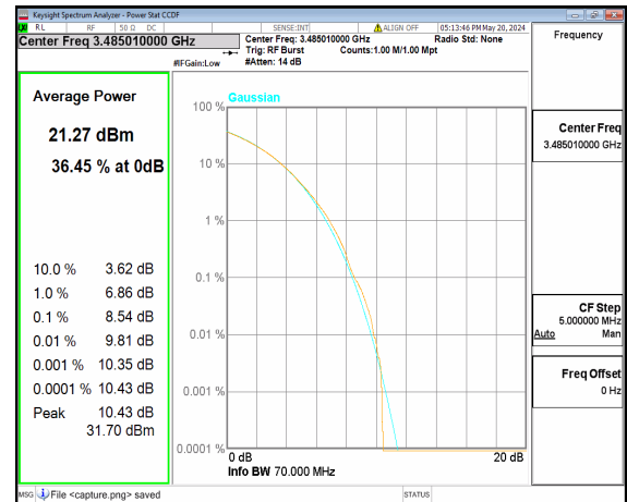
n77(3450-3550MHz) 70M CP-OFDM 256QAM Outer_Full Low
