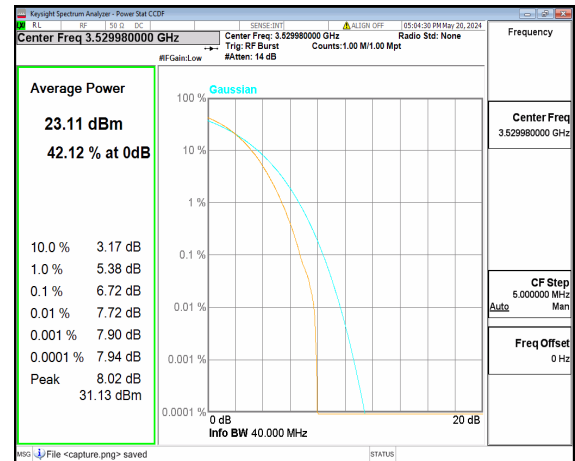
n77(3450-3550MHz) 40M DFT-s-OFDM 256QAM Outer_Full High
