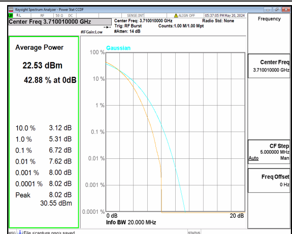
n77(3700-3980MHz) 20M DFT-s-OFDM 256QAM Outer_Full Low
