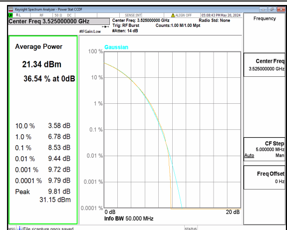
n77(3450-3550MHz) 50M CP-OFDM 256QAM Outer_Full High
