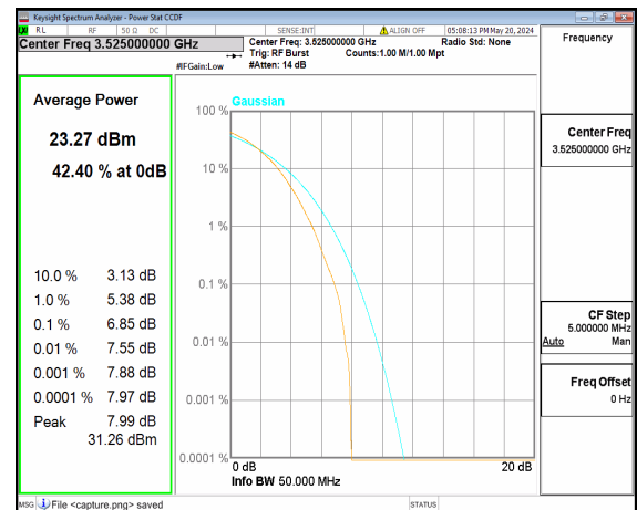
n77(3450-3550MHz) 50M DFT-s-OFDM 256QAM Outer_Full High
