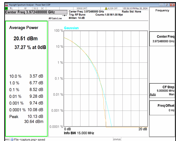
n77(3700-3980MHz) 15M CP-OFDM 256QAM Outer_Full High
