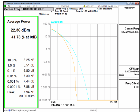
n77(3700-3980MHz) 10M DFT-s-OFDM 256QAM Outer_Full Mid
