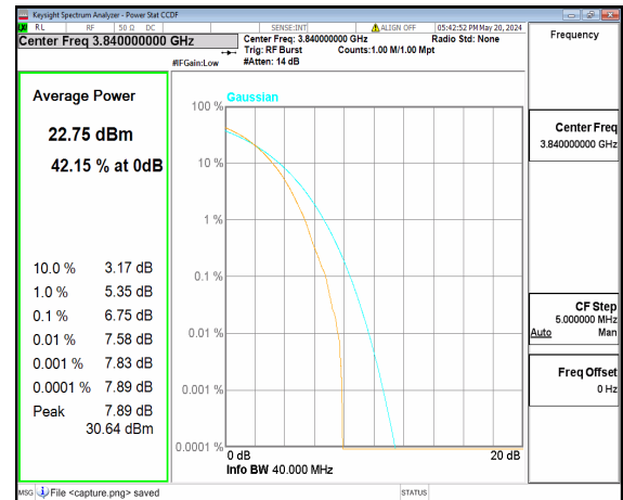
n77(3700-3980MHz) 40M DFT-s-OFDM 256QAM Outer_Full Mid
