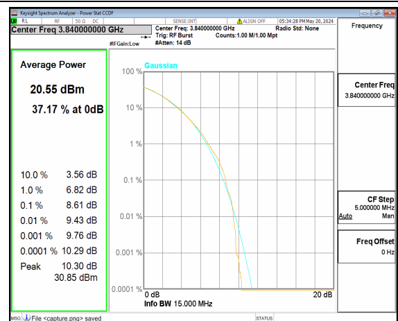
n77(3700-3980MHz) 15M CP-OFDM 256QAM Outer_Full Mid
