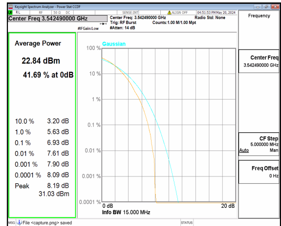
n77(3450-3550MHz) 15M DFT-s-OFDM 256QAM Outer_Full High
