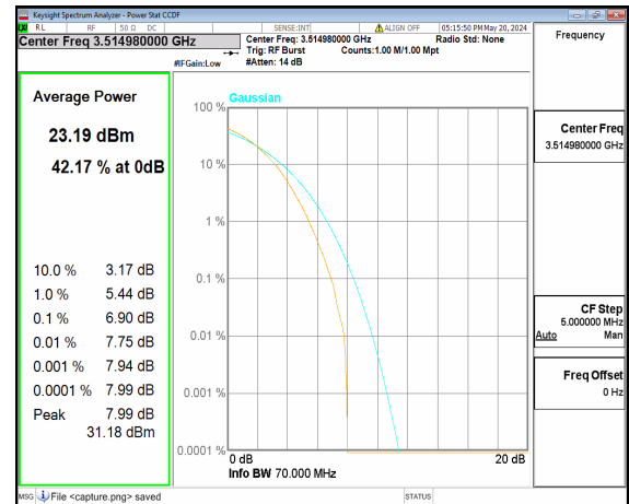
n77(3450-3550MHz) 70M DFT-s-OFDM 256QAM Outer_Full High
