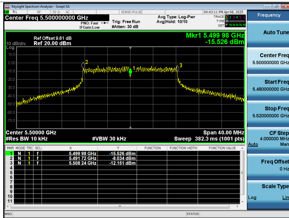
Freq. Stability 0C 12V a 5500MHz Ant1 0 Minutes
