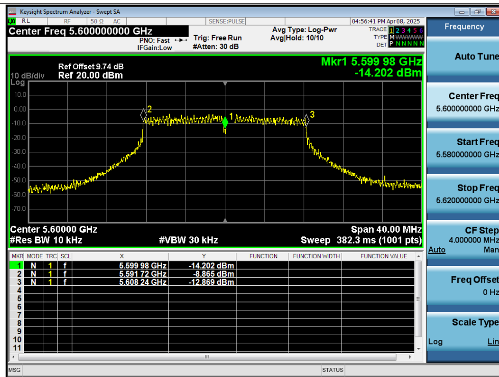
Freq. Stability 0C 12V a 5600MHz Ant1 0 Minutes
