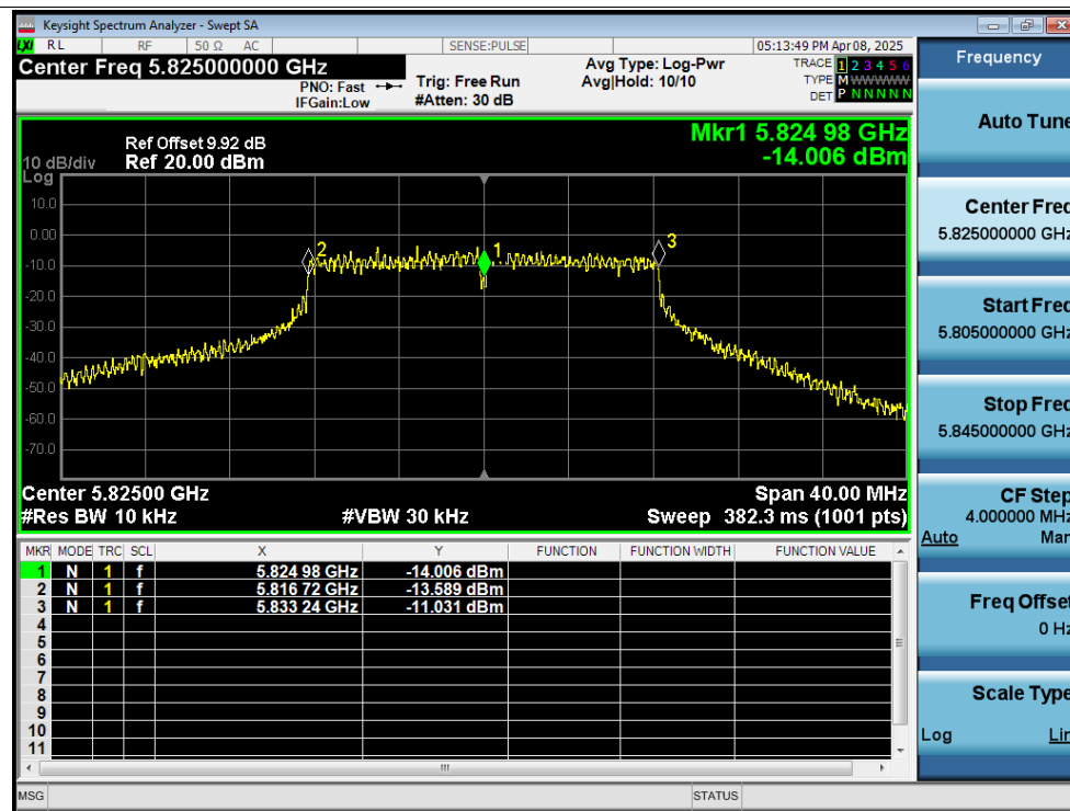
Freq. Stability 0C 12V a 5825MHz Ant1 0 Minutes
