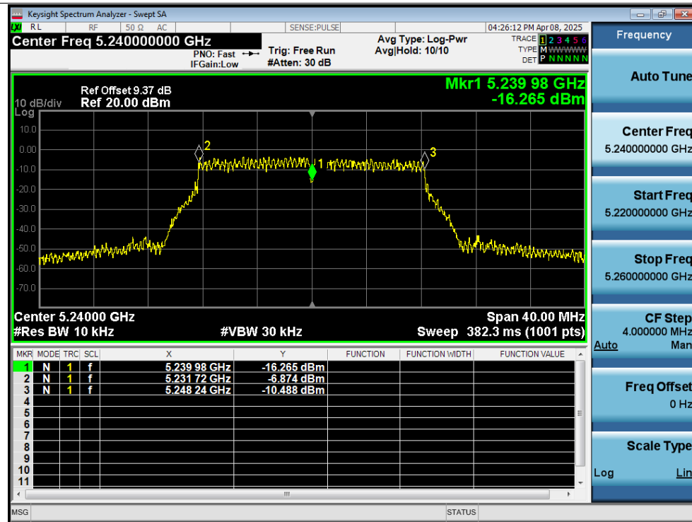
Freq. Stability 0C 12V a 5240MHz Ant1 0 Minutes
