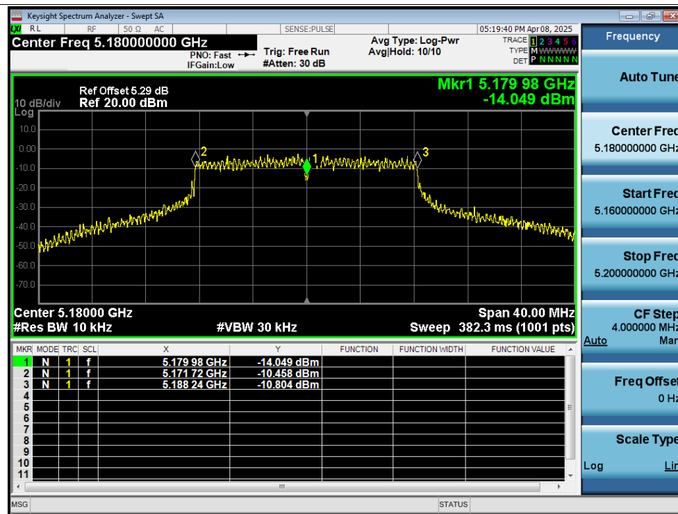
Freq. Stability 0C 12V a 5180MHz Ant2 0 Minutes
