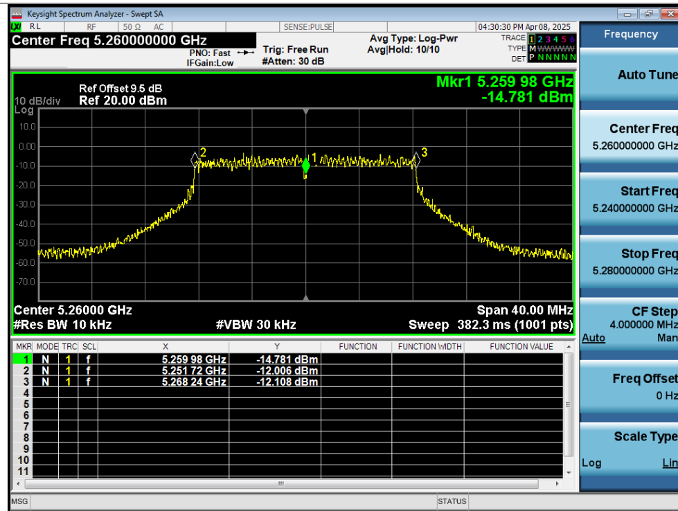
Freq. Stability 0C 12V a 5260MHz Ant1 0 Minutes
