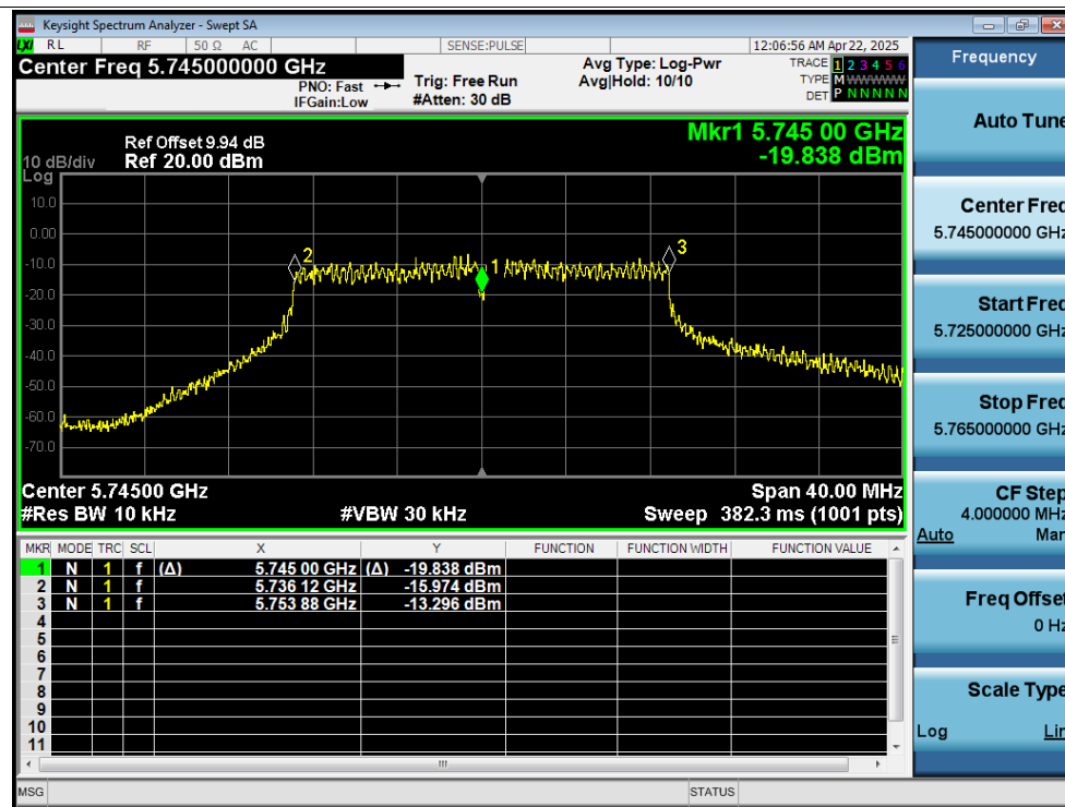
Freq. Stability 20C 12V n20 5745MHz Ant1 0 Minutes
