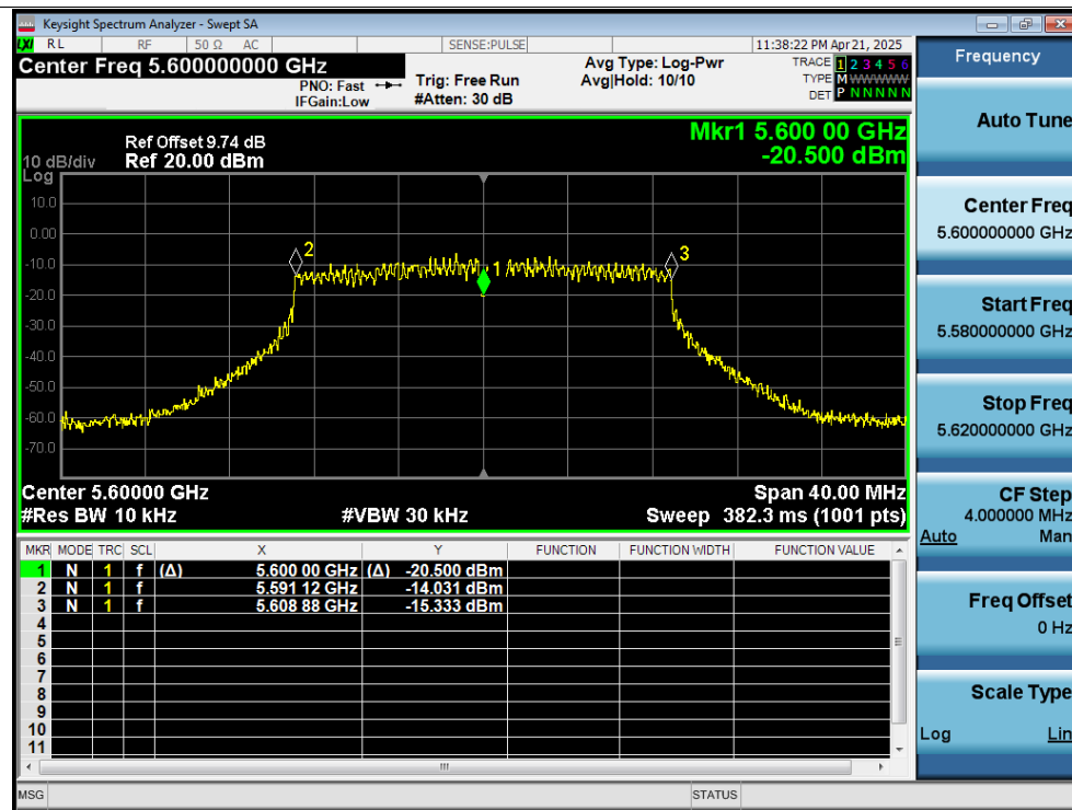
Freq. Stability 20C 12V n20 5600MHz Ant1 0 Minutes
