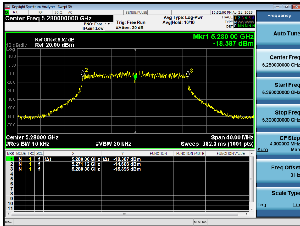
Freq. Stability 30C 12V n20 5280MHz Ant1 0 Minutes
