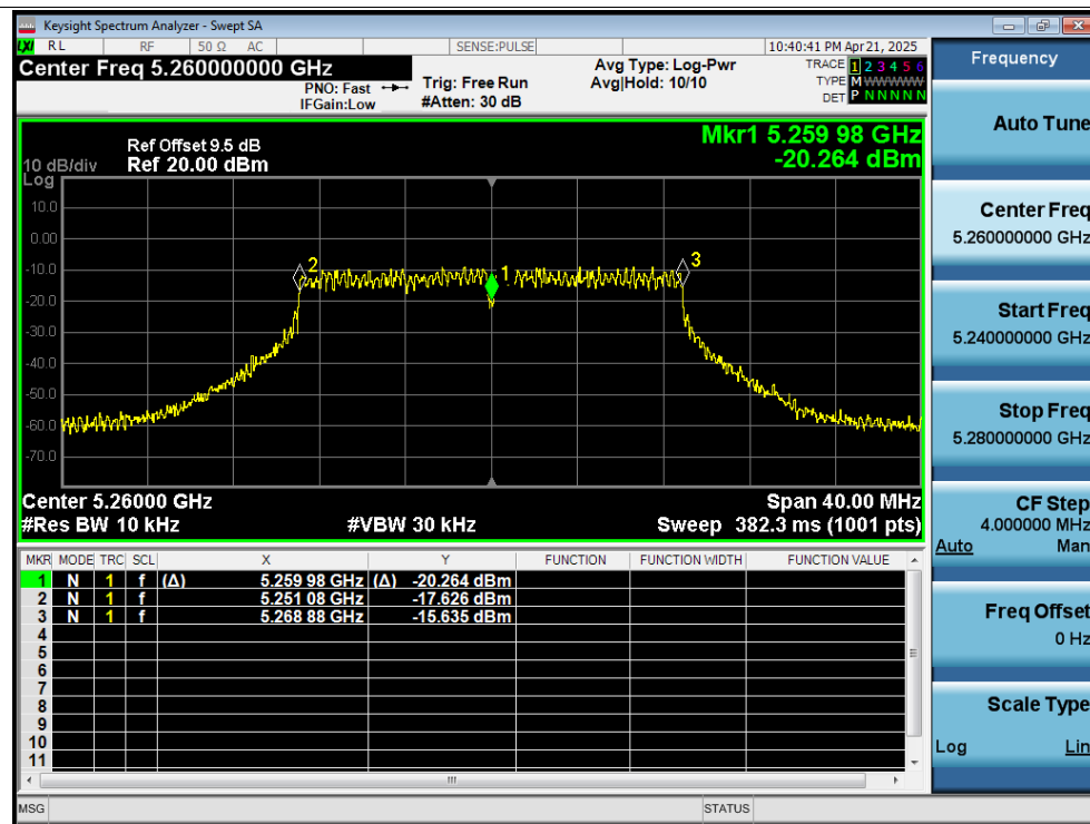
Freq. Stability 0C 12V n20 5260MHz Ant1 0 Minutes
