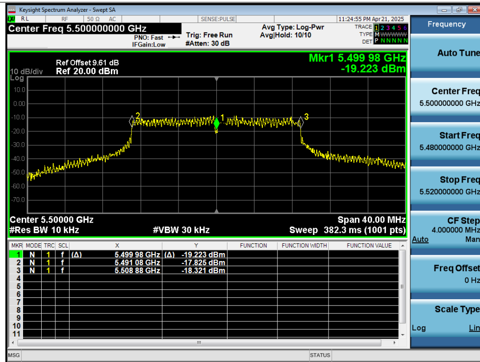
Freq. Stability 20C 12V n20 5500MHz Ant1 0 Minutes
