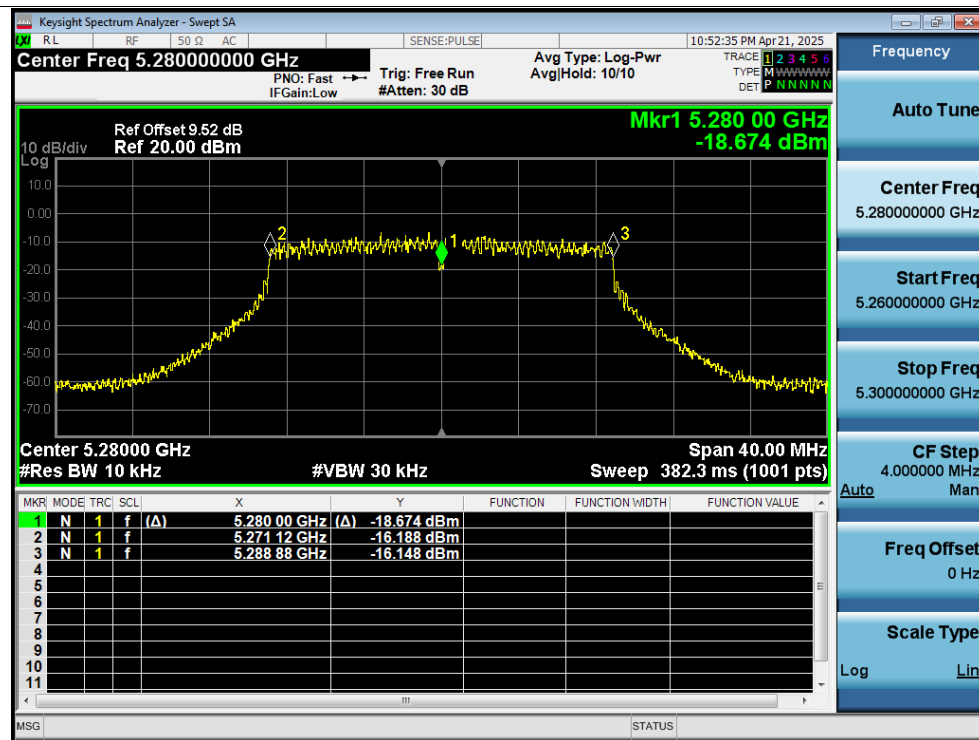
Freq. Stability 50C 12V n20 5280MHz Ant1 0 Minutes
