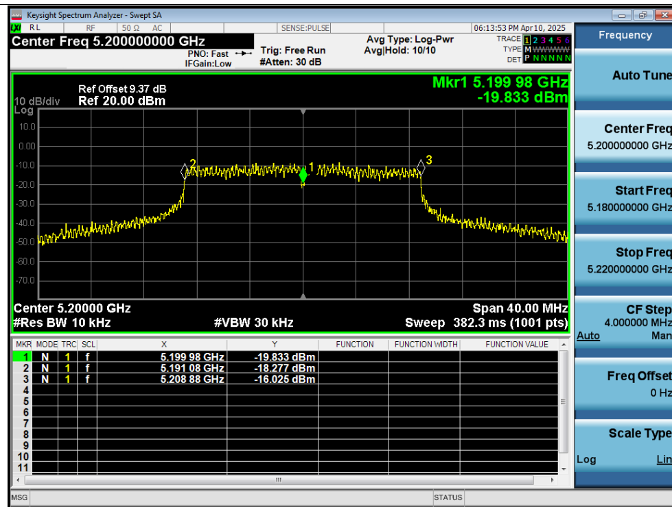
Freq. Stability 0C 12V n20 5200MHz Ant1 0 Minutes
