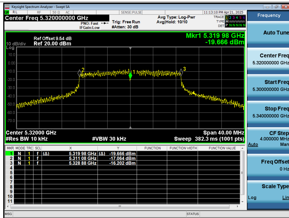
Freq. Stability 20C 12V n20 5320MHz Ant1 0 Minutes
