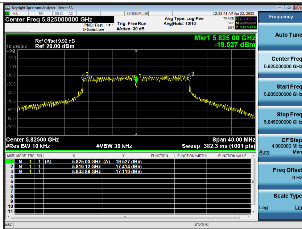
Freq. Stability 50C 12V n20 5825MHz Ant1 0 Minutes
