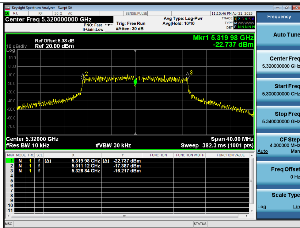
Freq. Stability 0C 12V n20 5320MHz Ant2 0 Minutes
