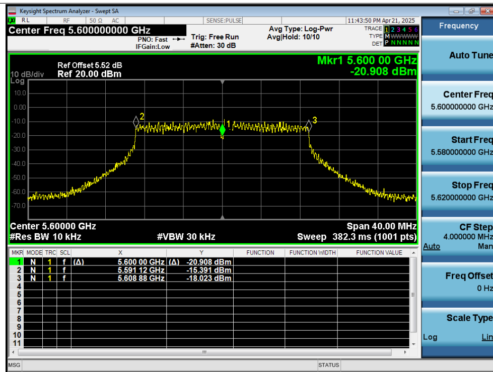
Freq. Stability 30C 12V n20 5600MHz Ant2 0 Minutes
