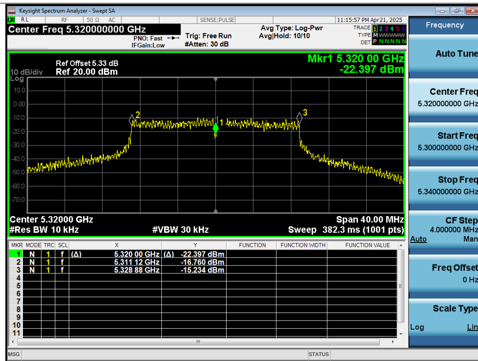
Freq. Stability 30C 12V n20 5320MHz Ant2 0 Minutes
