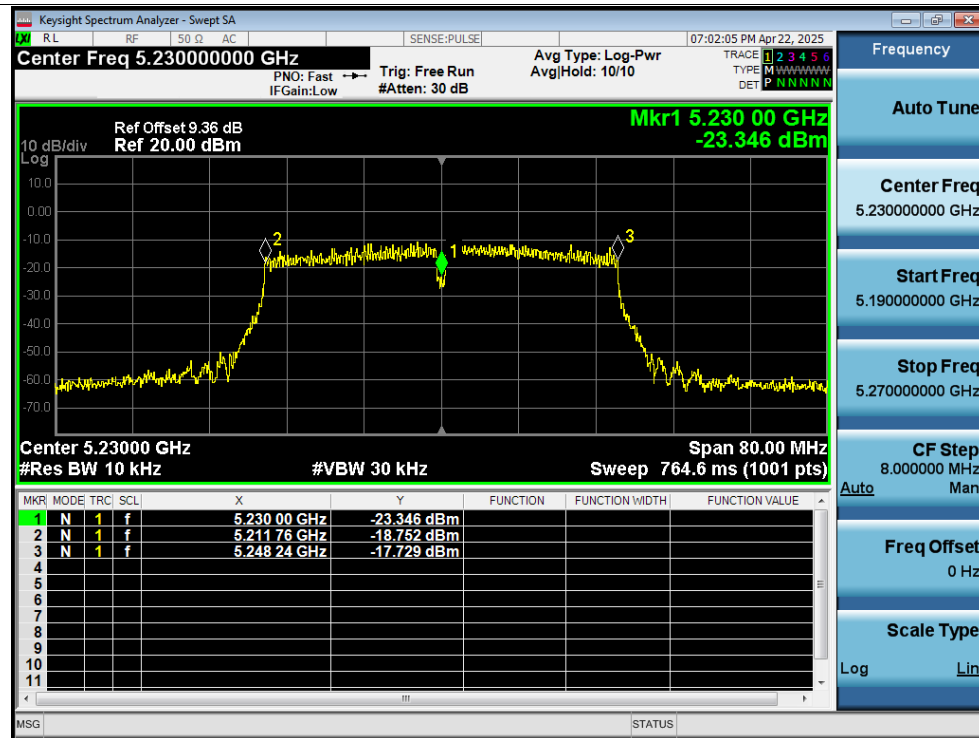
Freq. Stability 20C 13.8V n40 5230MHz Ant1 0 Minutes
