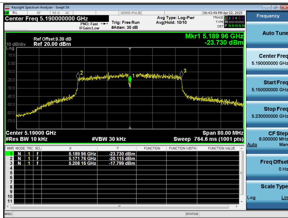
Freq. Stability 20C 13.8V n40 5190MHz Ant1 0 Minutes
