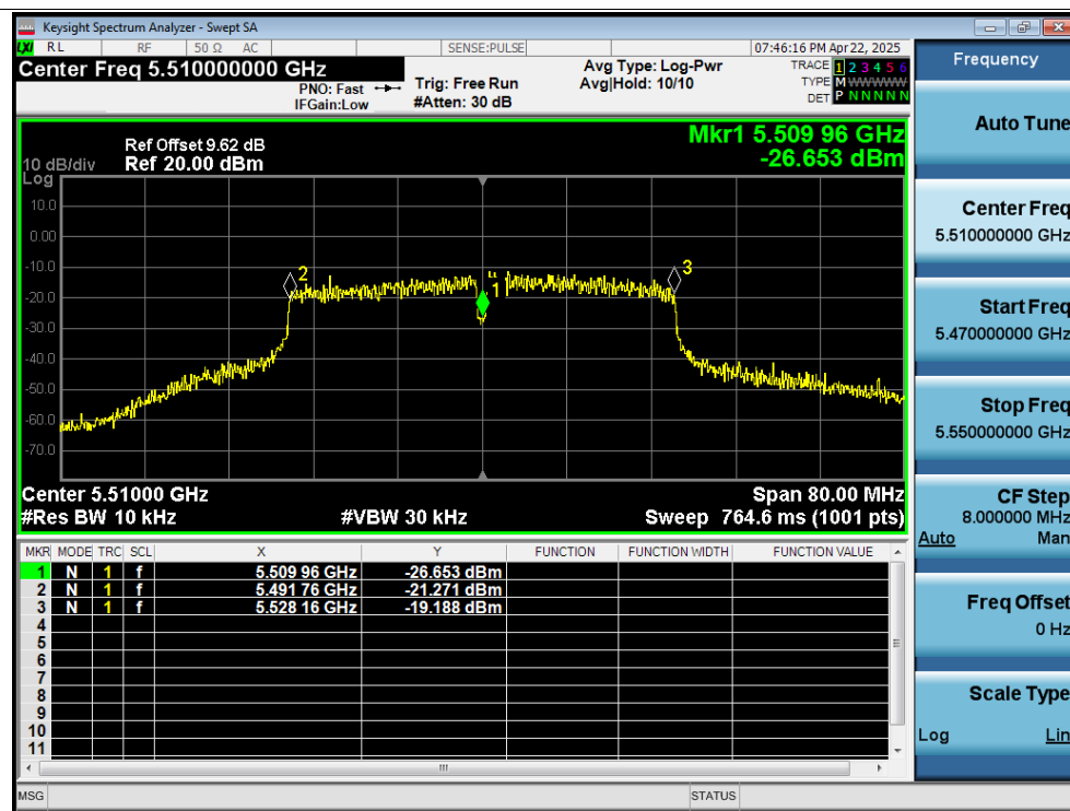
Freq. Stability 20C 13.8V n40 5510MHz Ant1 0 Minutes
