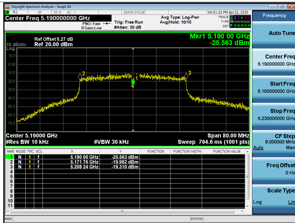
Freq. Stability 10C 12V n40 5190MHz Ant2 0 Minutes
