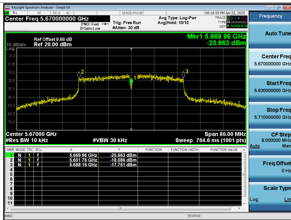
Freq. Stability 40C 12V n40 5670MHz Ant1 0 Minutes
