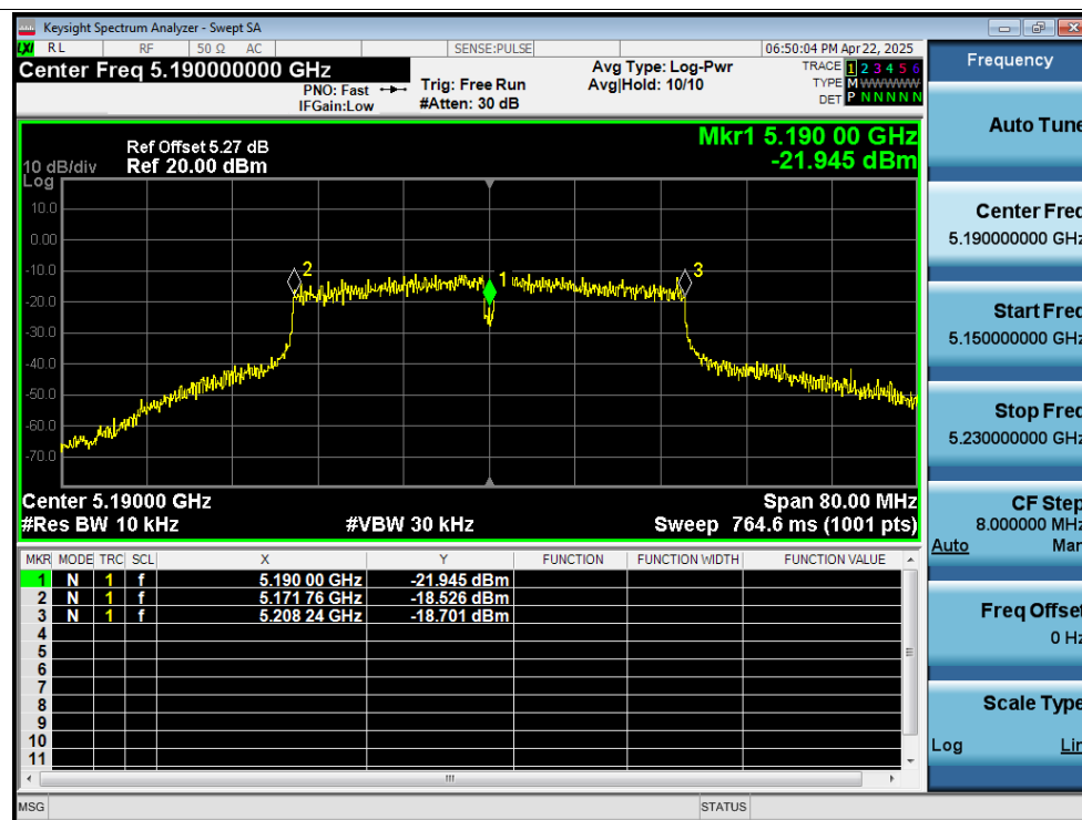
Freq. Stability 20C 10.2V n40 5190MHz Ant2 0 Minutes
