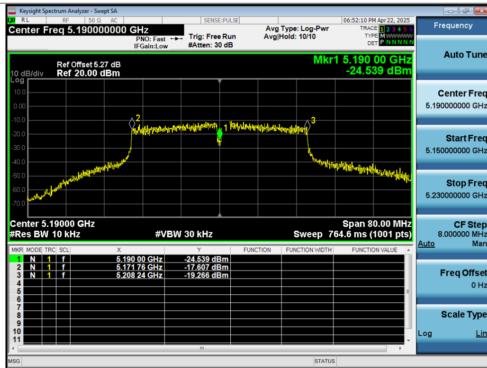
Freq. Stability 40C 12V n40 5190MHz Ant2 0 Minutes
