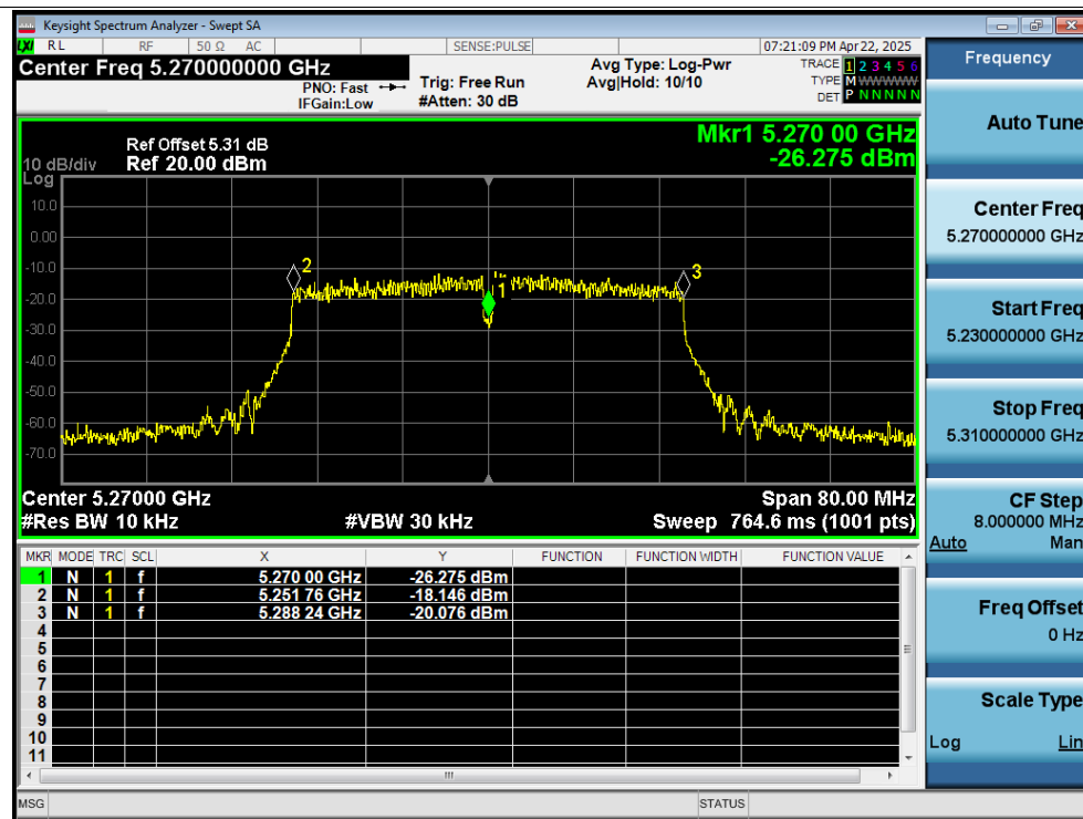
Freq. Stability 20C 10.2V n40 5270MHz Ant2 0 Minutes
