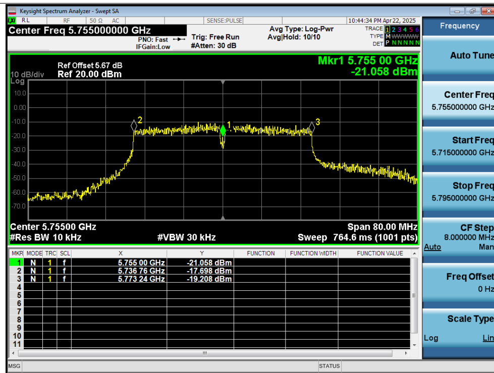
Freq. Stability 20C 13.8V ac40 5755MHz Ant2 0 Minutes
