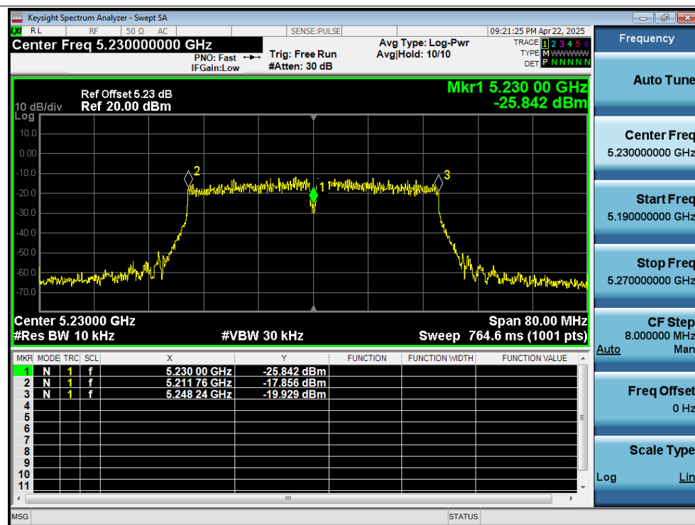
Freq. Stability 20C 13.8V ac40 5230MHz Ant3 0 Minutes
