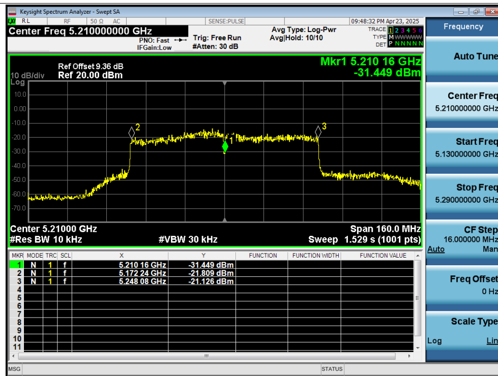
Freq. Stability -10C 12V ac80 5210MHz Ant1 0 Minutes
