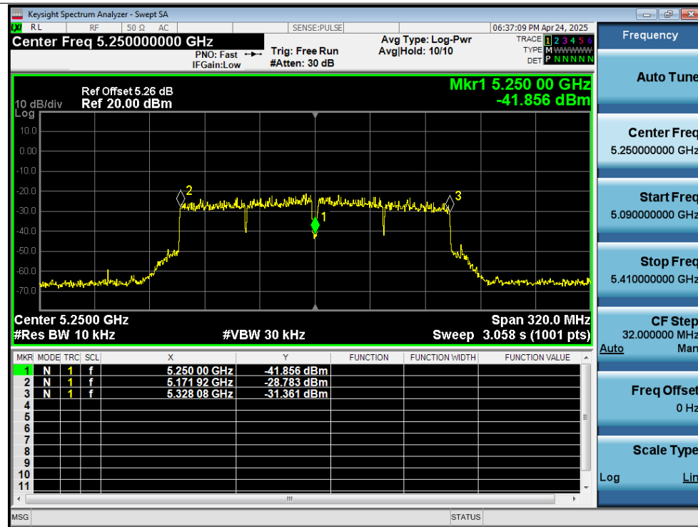
Freq. Stability 10C 12V ac160 5250MHz Ant3 0 Minutes
