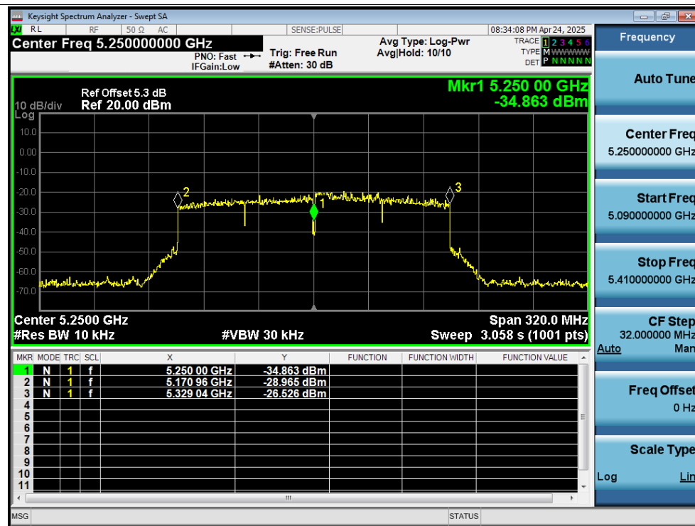
Freq. Stability 10C 12V ax160 5250MHz Ant2 0 Minutes
